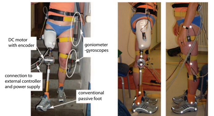
Fig. 1. Experimental Setup (left) and marker placement for gait analysis (right).
