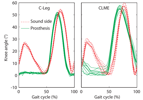
Fig. 4. Knee angle trajectories during treadmill walking with the C-Leg (left) and with a CLME-controlled active knee joint (right). Sound and prosthetic knee joint angles (dashed and solid lines, respectively) are normalized and plotted over multiple steps
