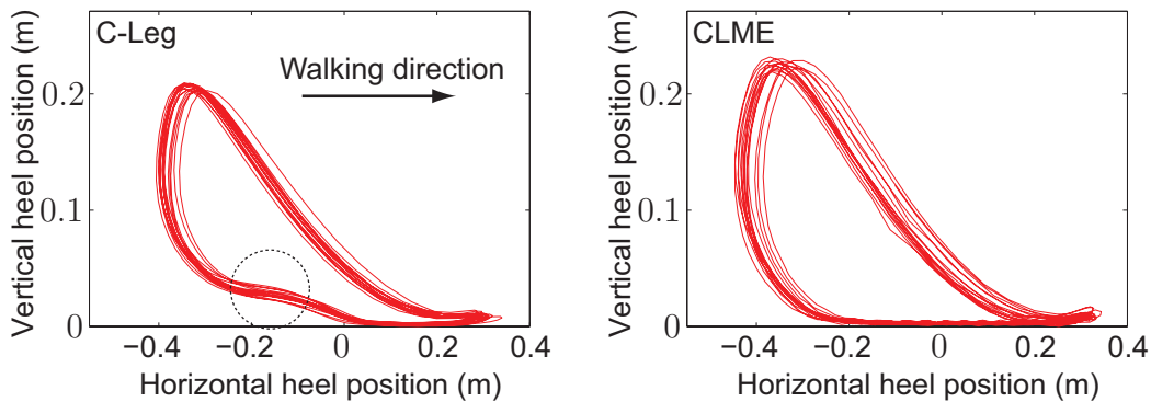
Fig. 3. Cartesian trajectory of the sound leg’s heel during treadmill walking with the C-Leg (left) and with a CLME-controlled active knee joint (right). Vaulting can be observed with the C-Leg.
