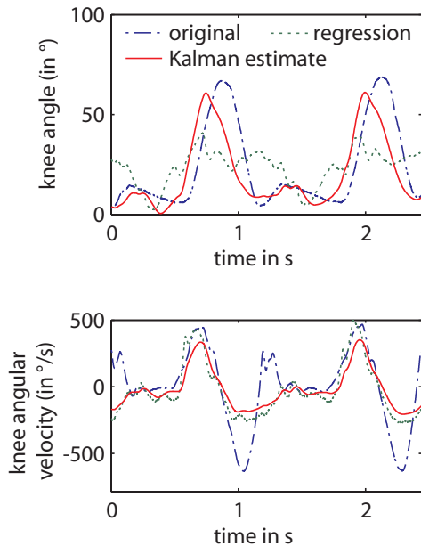
Fig. 2. Theoretical estimation accuracy when applying the regression and filtering to the off-line stored gait data of the non-impaired reference subject.
