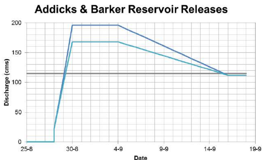
Figure 4.10. Approximate release rates (m 3 /s) from Addicks and Barker Reservoirs as reported by USACE starting on August 28. Release rates are reported to have peaked at about 200m 3 /s and 170 m 3 /s, respectively. Reduction of releases were reported as of September 4, however, the rate of release during the period between September 4 and 17 is unknown. By September 17, releases had been reduced to 115m 3 /s.
