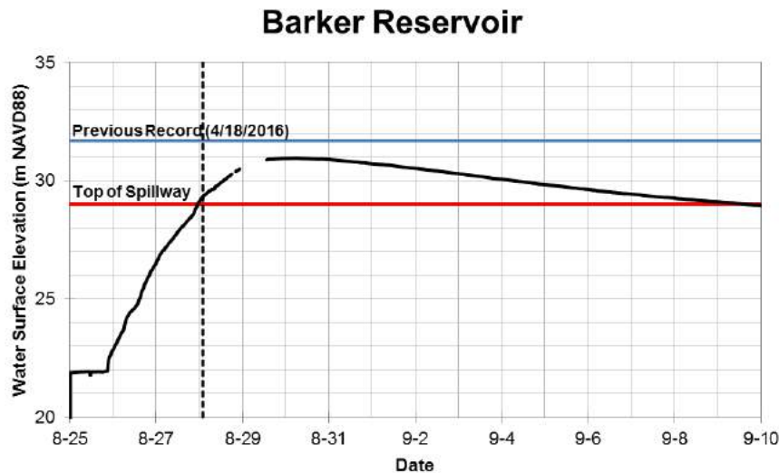
Figure 4.9b. Water levels (m NAVD88) in (a) Addicks (USGS 8073000) and (b) Barker (USGS 8072500) reservoirs between August 25 and September 10, 2017. The tops of the spillways are at 31.2 and 29.0 m, respectively. The previous record maximum water elevations reached during the Tax Day Flood (2016) are also shown.
