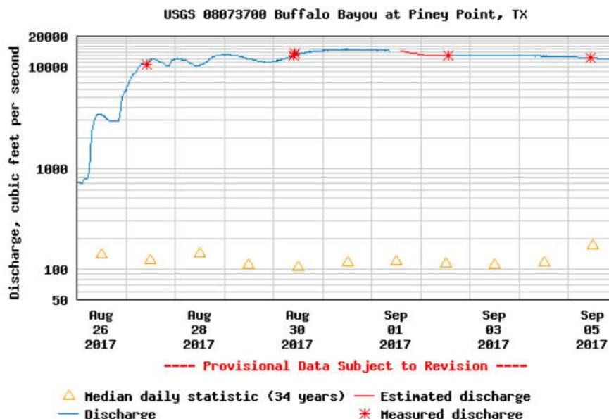
Figure 4.13: Discharge through Buffalo Bayou expressed in cubic feet per second (cfs). Included are the median daily discharge rates, which fluctuate between 100 and 1000 cfs
