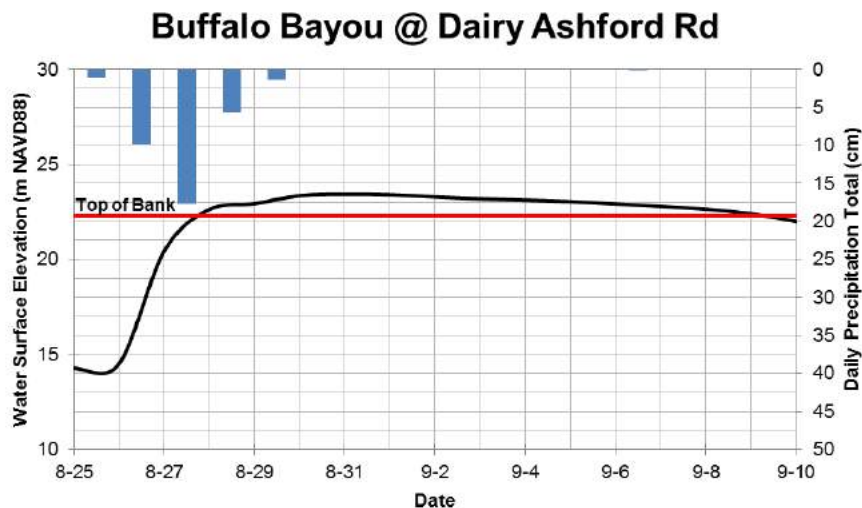
Figure 4.11. Water levels at Dairy Ashford Road, in Buffalo Bayou, between August 26 and August 29.
