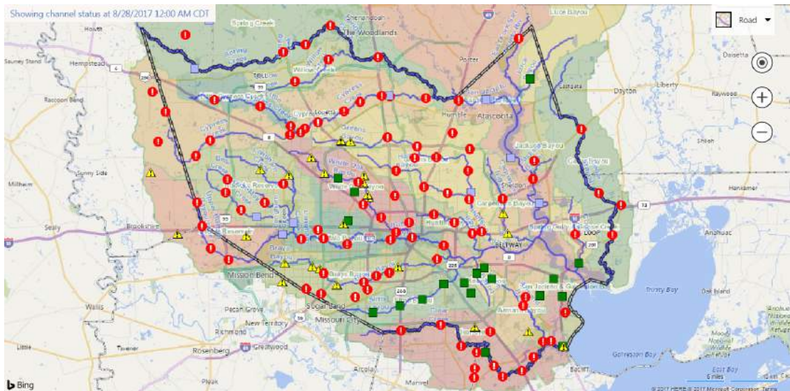
Figure 4.5. Status of the HCFCF stream gages as of August 28, 2017 12:00 AM (CDT). Locations marked in red are out of bank and locations in yellow are near the top of bank. Figure courtesy of https://www.harriscountyfws.org/ .
