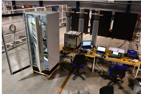
150kV LPIT setup at KEMA Labs
