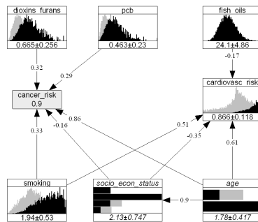
Figure 7. Conditionalised BBN for cancer\_risk = 0.9 .
