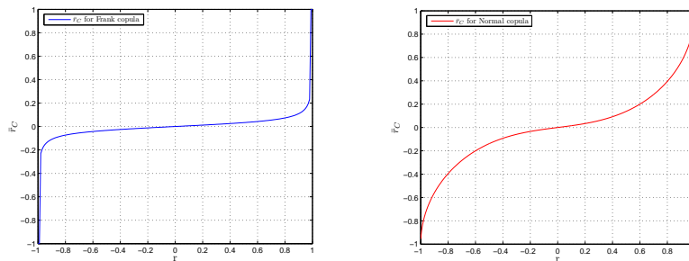
(a) p_{1+} = p_{+1} = p_{3+} = p_{+3} = 0.01, p_{2+} = p_{+2} = 0.98 . The joint distribution is constructed using Frank's copula. (b) p_{1+} = p_{+1} = p_{3+} = p_{+3} = 0.01, p_{2+} = p_{+2} = 0.98 . The joint distribution is constructed using the Normal copula.
