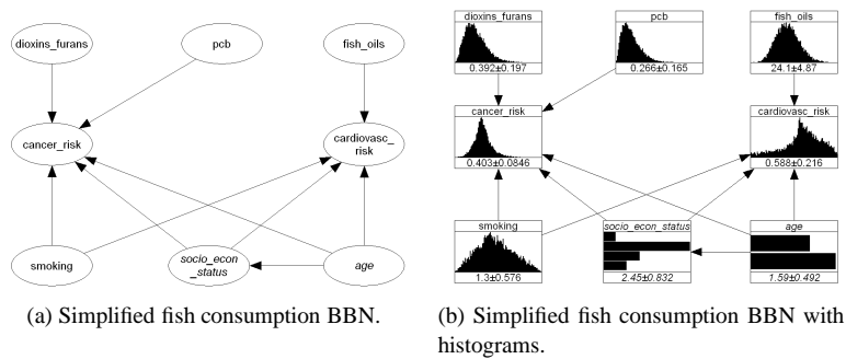
Figure 5. Simplified Bayesian Belief Net for fish consumption risks.
