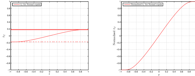
(a) The relation between r and \bar{r}_C , for X and Y , with not uniform, not equal, not "complementary" marginal distributions. (b) The relation between r and the normalised \bar{r}_C , for X and Y , with not uniform, not equal, not "complementary" marginal distributions.
