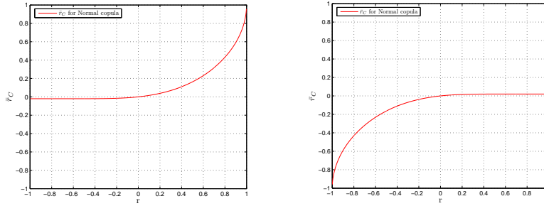
(a) p_{1+} = p_{+1} = p_{2+} = p_{+2} = 0.01, p_{3+} = p_{+3} = 0.98 . (b) p_{2+} = p_{+3} = p_{+1} = p_{+2} = 0.01, p_{1+} = p_{+3} = 0.98 .
