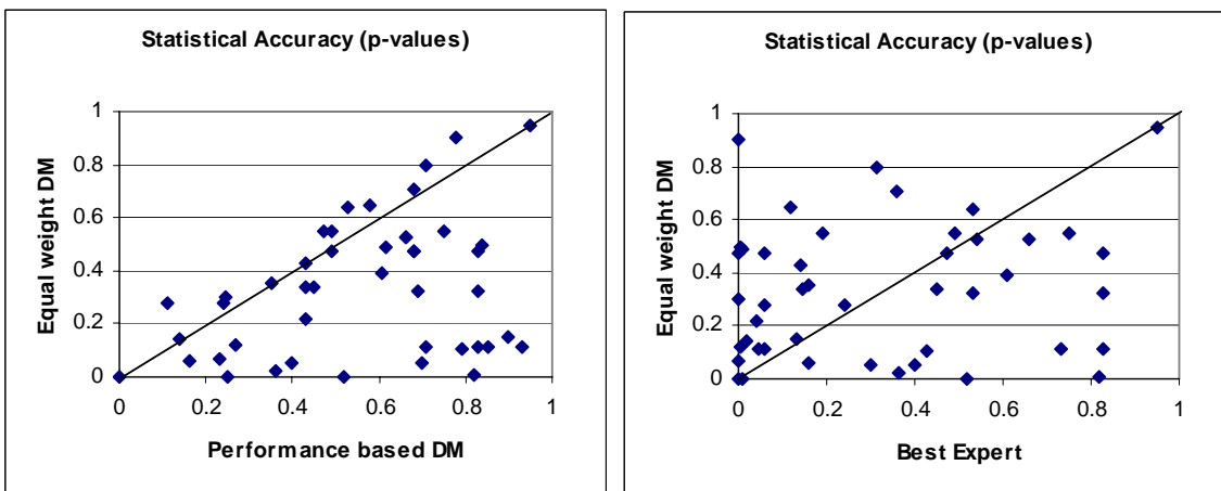
Figure 2 Calibration (p-values) and Information scores of Equal weight DM, Performance-based DM and best expert
