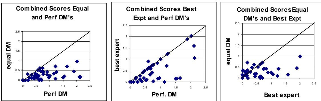
Figure 1. Combined scores of Equal weight DM, Performance-based DM and Best Expert
