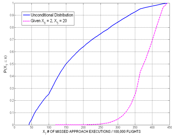
Figure 5.7: Cumulative Distribution function of X_7 and X_7|X_6 = 2 \text{ Nm} and X_5 = 20 \text{ Kt} .
