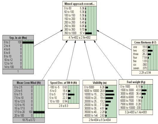
Figure 5.5: Conditional Distribution of Missed Approach Executions per 100,000 flights given X_6 \in (0, 2) Nm and X_5 \in (17.5, 20) Kt.
