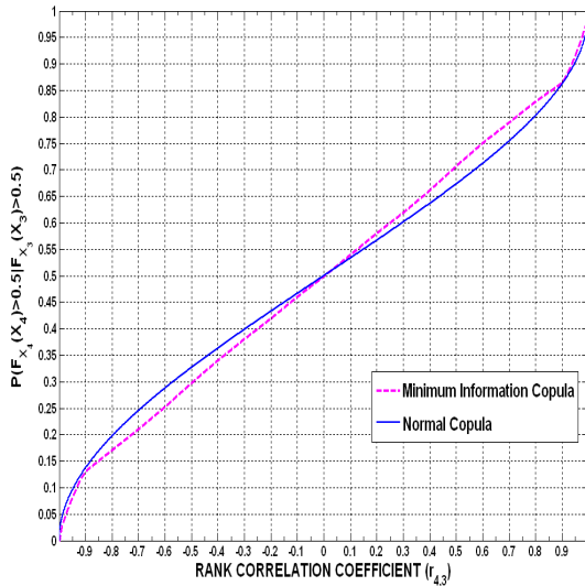
Figure 4.1: Relationship between P(F_{X_4}(X_4) \geq 0.5 | F_{X_3}(X_3) \geq 0.5) and r_{4,3} for normal and minimum information copula.
