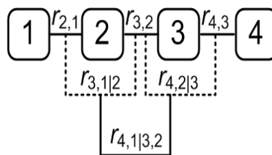
Figure 3.1: D-Vine on 4 variables with (conditional) rank correlations assigned to its edges.
