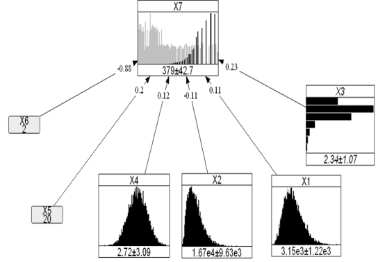
Figure 5.6: Conditional Distribution of Missed Approach Executions per 100,000 flights given X_6 = 2 Nm and X_5 = 20 Kt .
