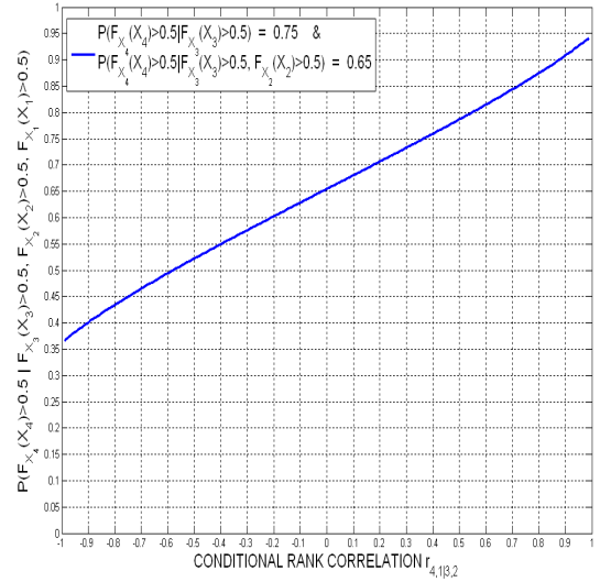
Figure 4.4: Relationship between P(F_{X_4}(X_4) \geq 0.5 | F_{X_3}(X_3) \geq 0.5, F_{X_2}(X_2) \geq 0.5, F_{X_1}(X_1) \geq 0.5) and the Rank Correlation Coefficient r_{4,1|3,2} for the four variate standard normal distribution.
