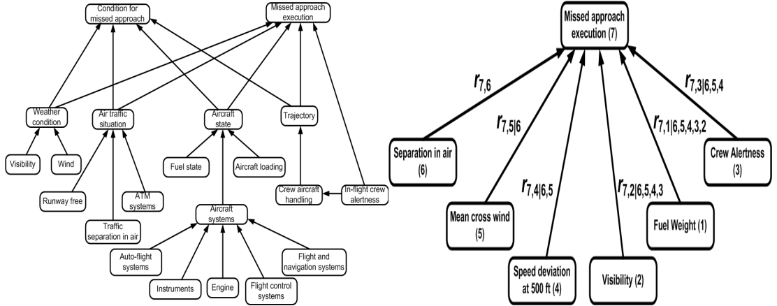
Figure 5.1: Original BBN of the Missed Approach Model.
