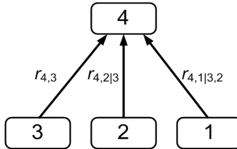
Figure 3.2: A simple example of BBN on 4 Variables.
