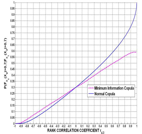
Figure 4.2: Relationship between P(F_{X_4}(X_4) \geq 0.7 | F_{X_3}(X_3) \geq 0.7) and r_{4,3} for normal and minimum information copula.
