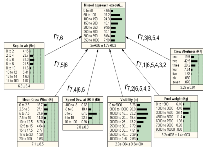
Figure 5.3: Discretized BBN of the Missed Approach Model with continuous quantities in Netica.
