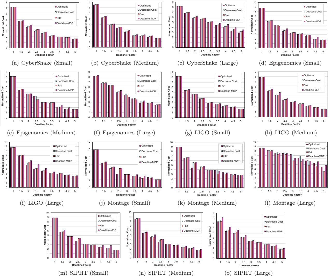
Figure 4: Normalized Cost of scheduling workflows with the PCP and Deadline-MDP algorithms
