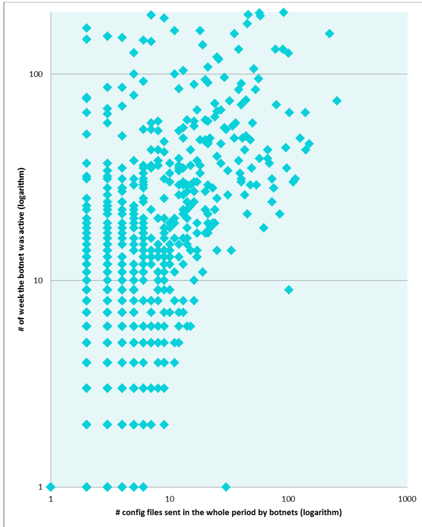
FIGURE 35- BOTNETS LIFESPAN VS. ACTIVITY (IN TERMS OF NUMBER OF CONFIG FILES THEY SENT)
