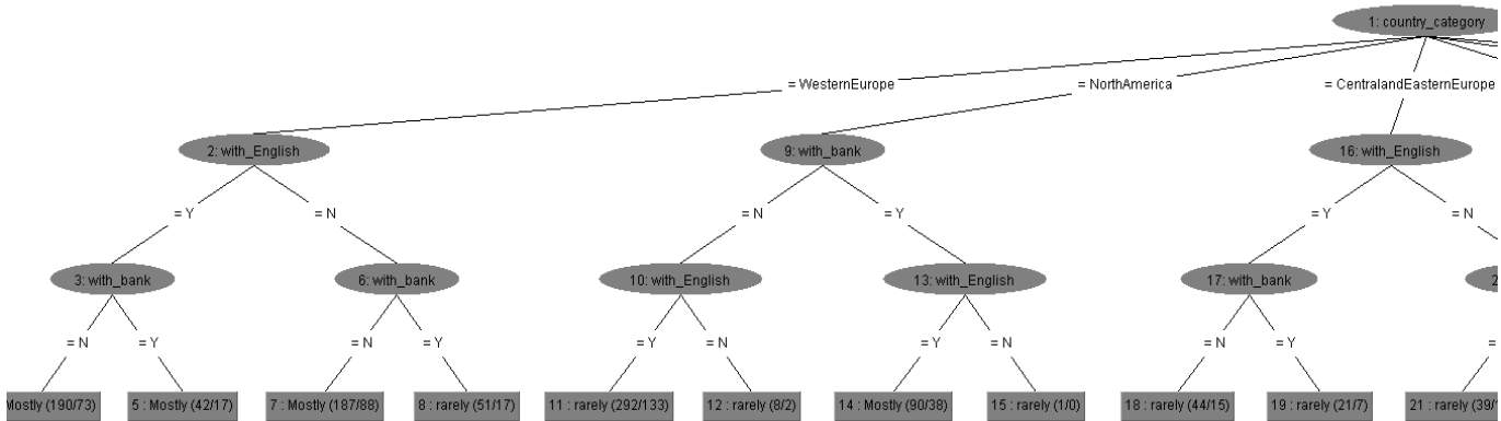
FIGURE 82 – VISUAL TREE (LEFT PART)
