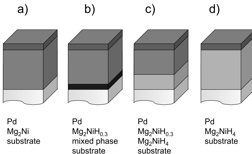
Figure 3.5: Schematic representation of the hydrogenation process of Mg 2 Ni covered with Pd (a). Mg 2 Ni absorbs hydrogen up to a concentration of Mg 2 NiH 0.3 . b) The nucleation of Mg 2 NiH 4 starts in a thin layer at the substrate-film interface. c) When this ~30-nm thick layer is completely converted into Mg 2 NiH 4 the hydrogenated layer starts to grow at the expense of the metallic layer towards the Pd top layer. This means that the hydrogenation process causes a self-organized double layering. d) Finally, the entire layer is hydrogenated.
