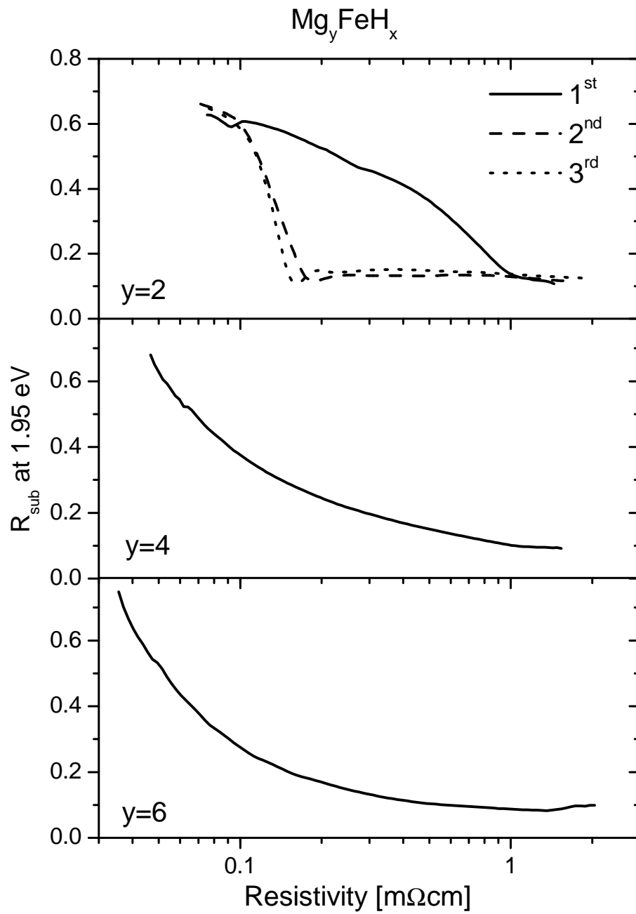
Figure 3.17: Reflection through the substrate R_{sub} at \hbar\omega = 1.95 eV of \text{Mg}_y\text{FeH}_x with y = 2, 4, 6 for the first three hydrogenation cycles. The 200 nm \text{Mg}_y\text{Fe} films are capped with 5 nm Pd. For y = 4, 6 dehydrogenation in air was not possible even when heated up to 95 °C.
