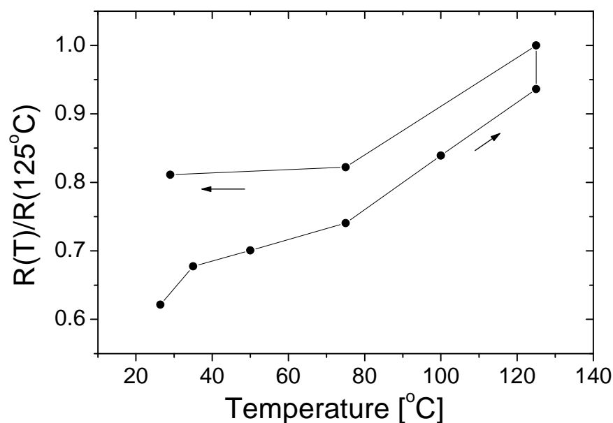
Figure 4.17: Average normalized reflection signal (channel green and blue) of the RGB camera at various temperatures through the substrate of an all-solid-state thermochromic device with \text{Mg}_2\text{Ni} (100 nm) as the switchable mirror, Pd (1500 nm) as the H reservoir layer and Cu as the H impermeable layer.
