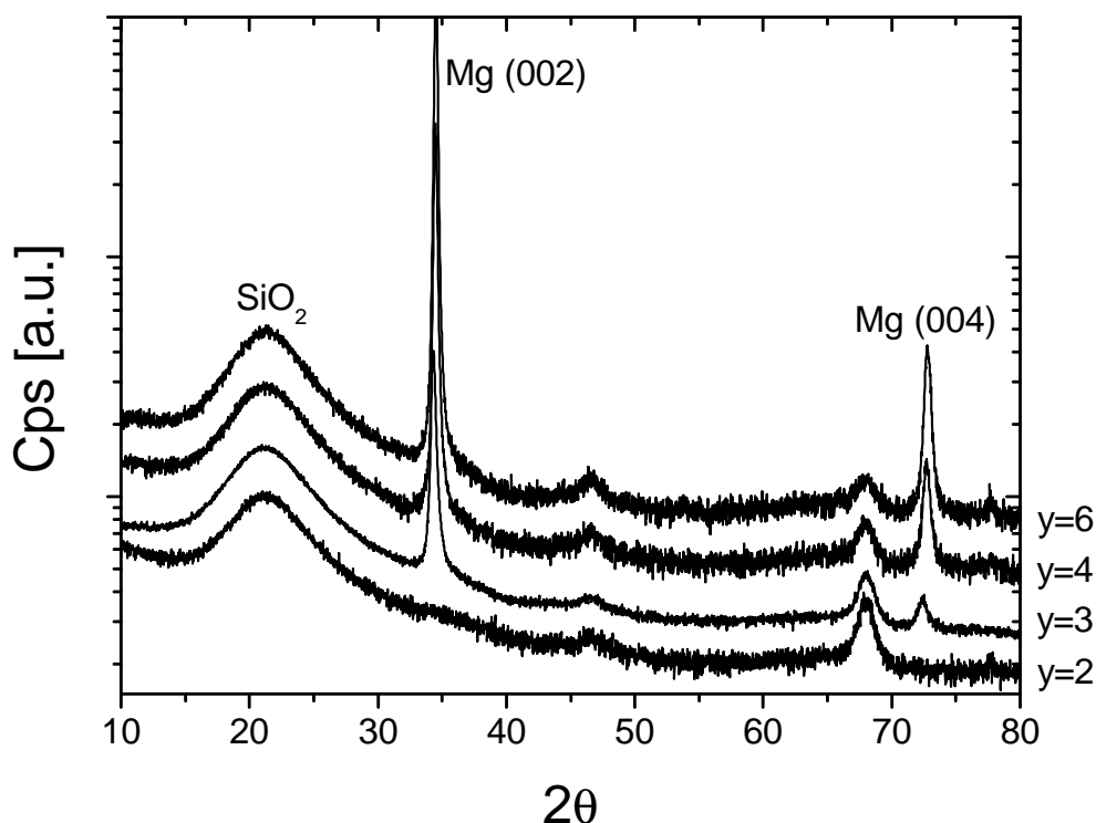
Figure 3.22: X-ray diffraction spectra of 200-nm thick Mg_yCo ( y = 2, 3, 4, 6 ) samples. The different spectra have been shifted for clarity. We observe an increase of the peak height with increasing Mg-to-Co ratio for the (002) and (004) Mg peak and a decrease of the lattice spacing. The small peak at 2\theta = 46.5^\circ ( d = 1.95 \text{ \AA} ) is probably due to Mg_2Pd_5 (222).
