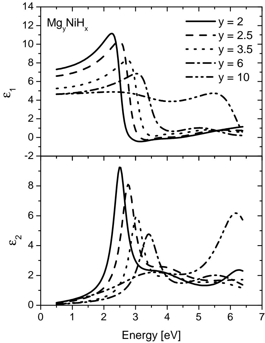
Figure 3.4: Fitted real \varepsilon_1 and imaginary \varepsilon_2 part of the dielectric functions of Mg_yNiH_x with y = 2, 2.5, 3.5, 6 and 10 [47].
