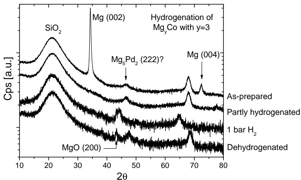
Figure 3.23: X-ray diffraction spectra of Mg_yCoH_x with y = 3 during hydrogenation. The Mg-peaks disappear and do not reappear after dehydrogenation. Two peaks shift to lower angles indicating hydrogen absorption. The MgO (200) peak appears during hydrogenation.
