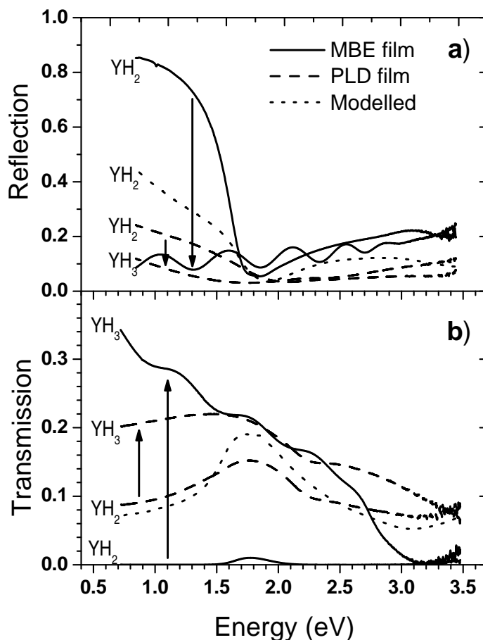
Figure 2.8: Comparison of the optical properties over a wide spectral range of the YH_2 and the YH_{3-\delta} phase for epitaxial PLD (70 nm) and MBE (150 nm) grown films. a) Reflection. b) Transmission. The finite transmission at energies larger than the yttrium band gap, E > E_g^{YH_3} , indicates the presence of secondary phases. An 70 nm thick modelled film of a Bruggeman mixture of 60% yttrium dihydride and 40% yttrium oxide covered by a 10 nm thick Pd layer is represented by the dotted line
