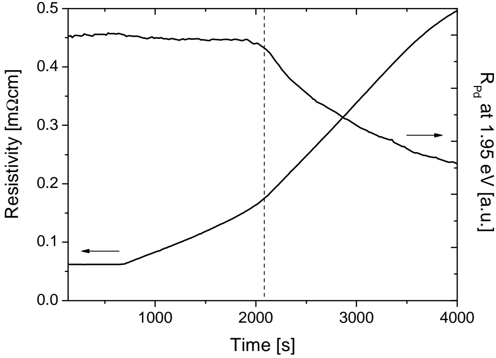
Figure 3.16: Resistivity and reflection R_{Pd} at \hbar\omega = 1.95 eV as a function of time for the first hydrogen loading at 5 mbar H_2 of a 200 nm Mg_yCo with y = 4 with 10 nm Pd on top. A change in the slope of the resistivity is observed around 2000 s simultaneously with the onset of the decrease of the Pd-side reflection R_{Pd} at constant H_2 pressure. This change of slope indicates the onset of homogeneously dispersed nucleation of Mg_2CoH_5 in the top metallic layer.
