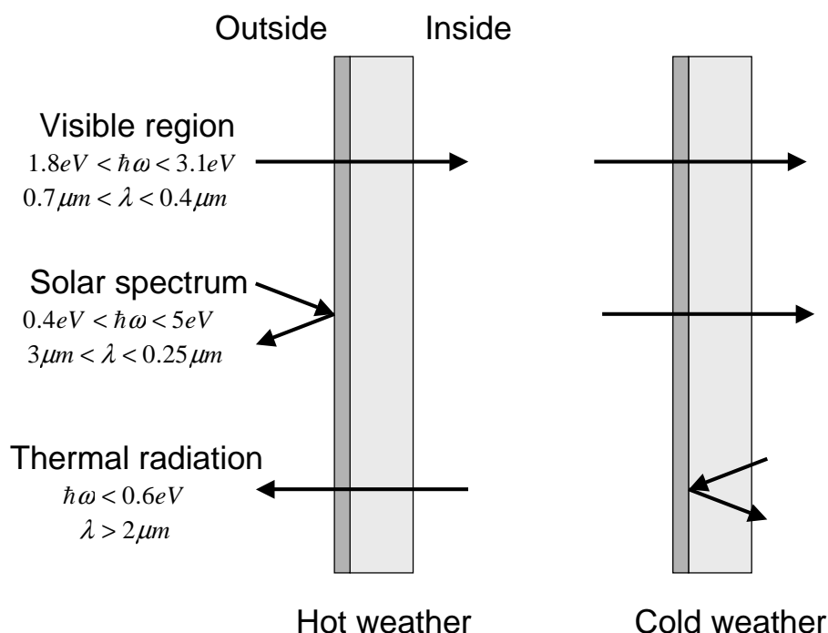
Figure 1.5: Desirable optical properties at various wavelengths during hot and cold weather. To maintain outward visibility, the smart window has to be transparent in the visible region at all times. Solar radiation should be reflected during hot weather and let through during cold days. For thermal radiation it is the other way around.
