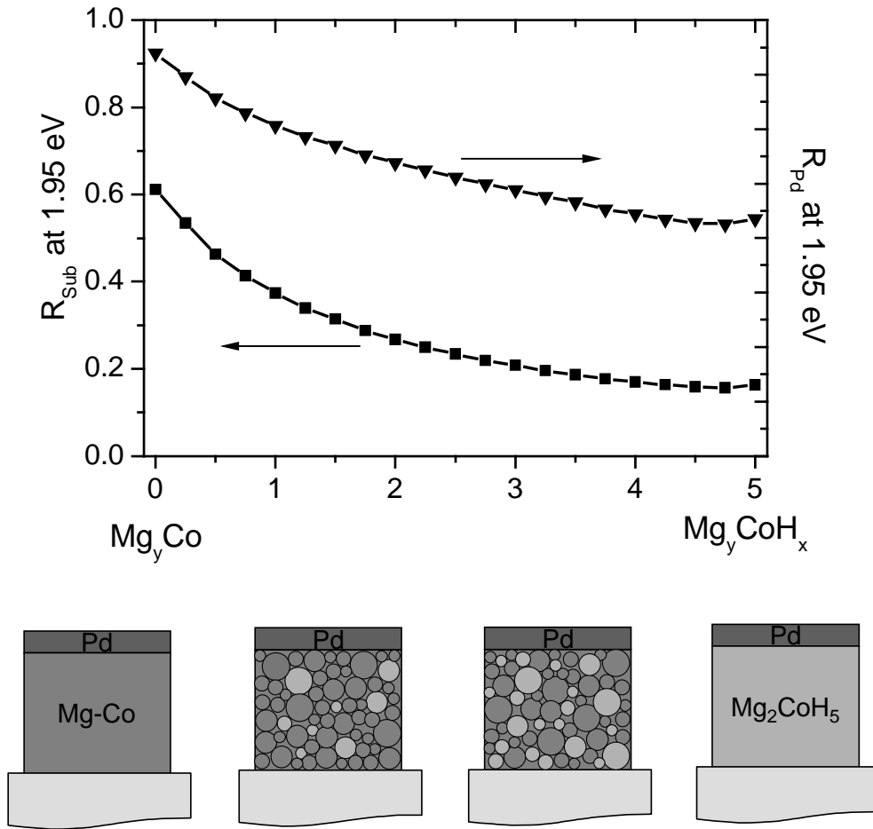
Figure 3.18: First model of the hydrogenation process of Mg_yCo with y = 2 of homogeneous nucleation throughout the film (see text).
