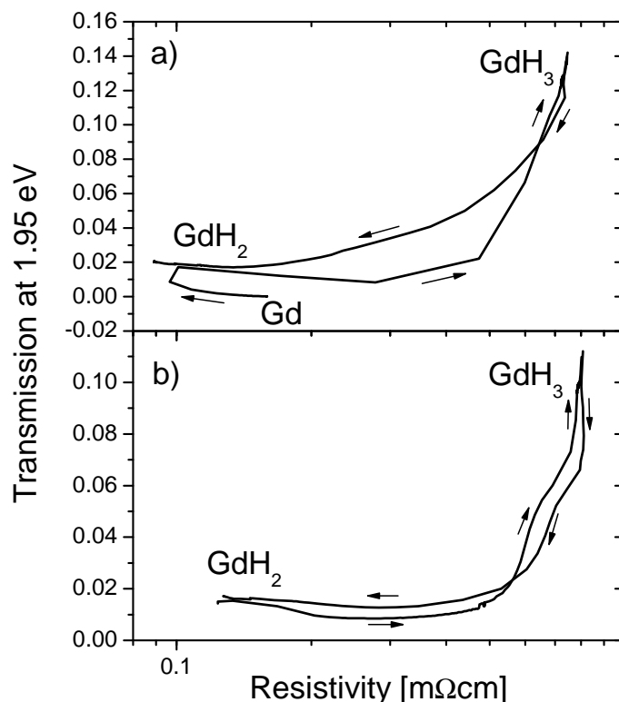
Figure 2.11: Transmission versus electrical resistivity during hydrogenation up to 1 bar H_2 at room temperature and dehydrogenation in air at 90^\circ C . a) Combining resistivity and transmission during hydrogenation and dehydrogenation reveals the presence or absence of hysteresis in switching for the Gd film deposited with the use of a clean target. a) Metallic Gd-film showing hysteresis. b) In-situ grown GdH_2 film with almost no hysteresis. Optical and RBS measurements show a decreased oxygen concentration as compared to the YH_2 films. The optical range has increased considerably.
