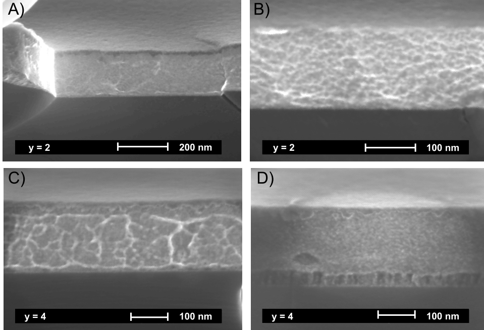
Figure 3.21: SEM micrographs of the cross section of 200 nm thick Mg_yCoH_x films deposited on a Si substrate and covered by 10 nm Pd. a) y = 2 , as-prepared, b) y = 2 , after three switching cycles c) y = 4 , as-prepared d) y = 4 , after three switching cycles. The film has not been dehydrogenated and there is probably some hydrogen left in the lower 40 nm. For y = 2 small grains of the order of \sim 10 nm are observed. We find that the grain size increases with increasing Mg-content. For y = 4 , the grain size decreased after the switching cycles. Note that the pictures have different scales. (RUG: B.J. Kooi and G.H. ten Brink)
