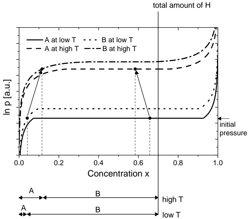
Figure 4.3: Schematic pressure-composition isotherms of metal hydrides A and B showing the hydrogen redistribution upon temperature increase in a closed system. In the example showed we have arbitrarily loaded the device with hydrogen to have x_A = 0.04 and x_B = 0.66 at low temperature. At a higher temperature these concentrations have changed to x_A = 0.12 and x_B = 0.58 . It is important to note, that the total amount of hydrogen stays constant.
