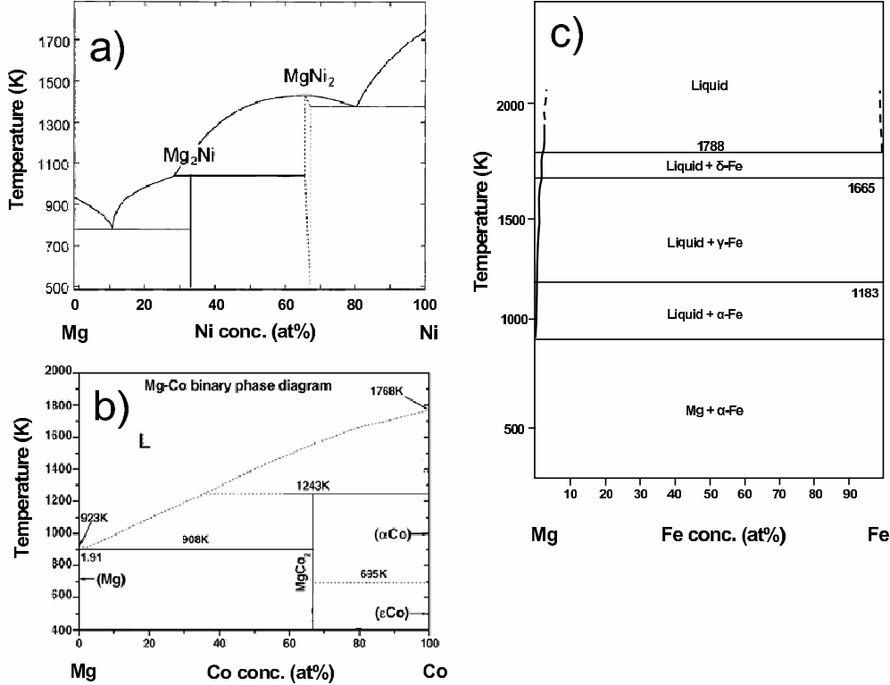
Figure 3.1: Temperature-composition metal phase diagrams of the binary systems for bulk materials of a) Mg-Ni [21] b) Mg-Co [22], Note, that the MgCo phase is not indicated in the phase diagram here [7, 8] and c) Mg-Fe [23]. Only for TM=Ni does a binary Mg-TM parent alloy exist with the same composition as in the ternary Mg_2TMH_x . For TM=Co two binary alloys exist with a different composition compared to the ternary alloy. The Mg-Fe system does not exhibit binary alloys.
