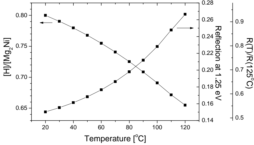
Figure 4.16: Calculated change in concentration in the \text{Mg}_2\text{NiH}_x layer of a 200 nm \text{Mg}_2\text{Ni}/3000 nm Pd bilayer as a function of temperature together with the accompanying change in normalized reflection at a photon energy of 1.25 eV as taken from [22]. Note that since the molar volume of Pd and \text{Mg}_2\text{Ni} is 8.56 and 31.2 \text{cm}^3 , respectively, and the amount of relevant H interstitial sites is 0.6 and 4, the ratio of the H interstitial sites in this case is N_{Pd}/N_{Mg_2Ni}=8.2
