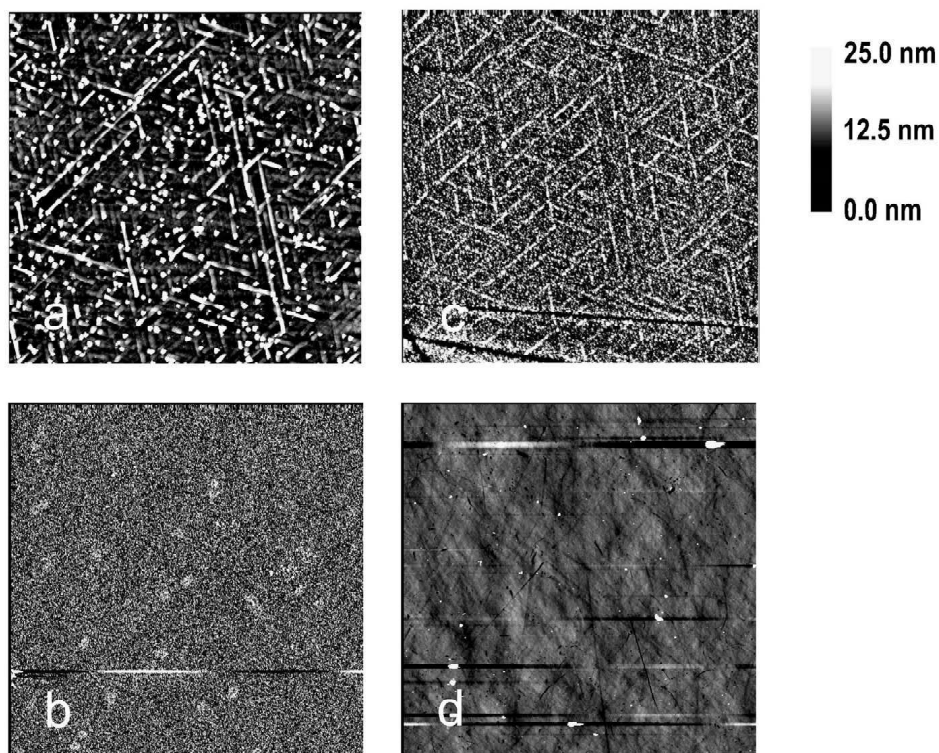
Figure 2.6: AFM tapping micrographs of \text{YH}_2 films. All images have the same height scale and have the same size (25x25 micrometers). a) Ex-situ hydrogenated epitaxial MBE film with typical ridge pattern. b) In-situ grown epitaxial PLD film with typical morphology. c) In-situ grown epitaxial PLD film. Ridges are only observed when using deposition temperatures above 500^\circ\text{C} . These ridges consist of elevated grains. d) In-situ grown nanocrystalline \text{YH}_2 film at room temperature on quartz. The surface has a flat and wavy appearance. The horizontal lines are artifacts caused by the large contrast in height of some particles on the film surface.
