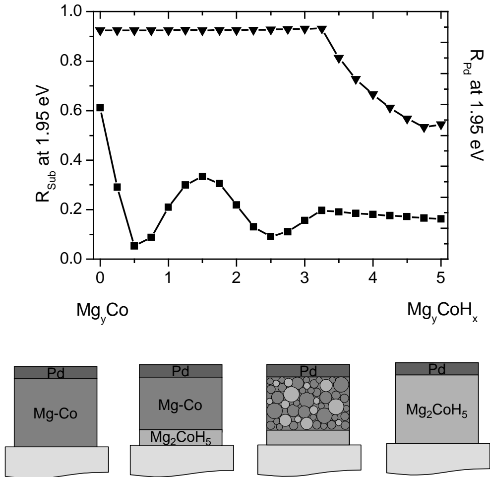
Figure 3.20: Third model of the hydrogenation process of \text{Mg}_y\text{Co} with y = 2 . This is a combination of the first (see Fig. 3.18) and second (see Fig. 3.19) models; a double layer formation evolves into homogeneous nucleation at intermediate hydrogen concentration.
