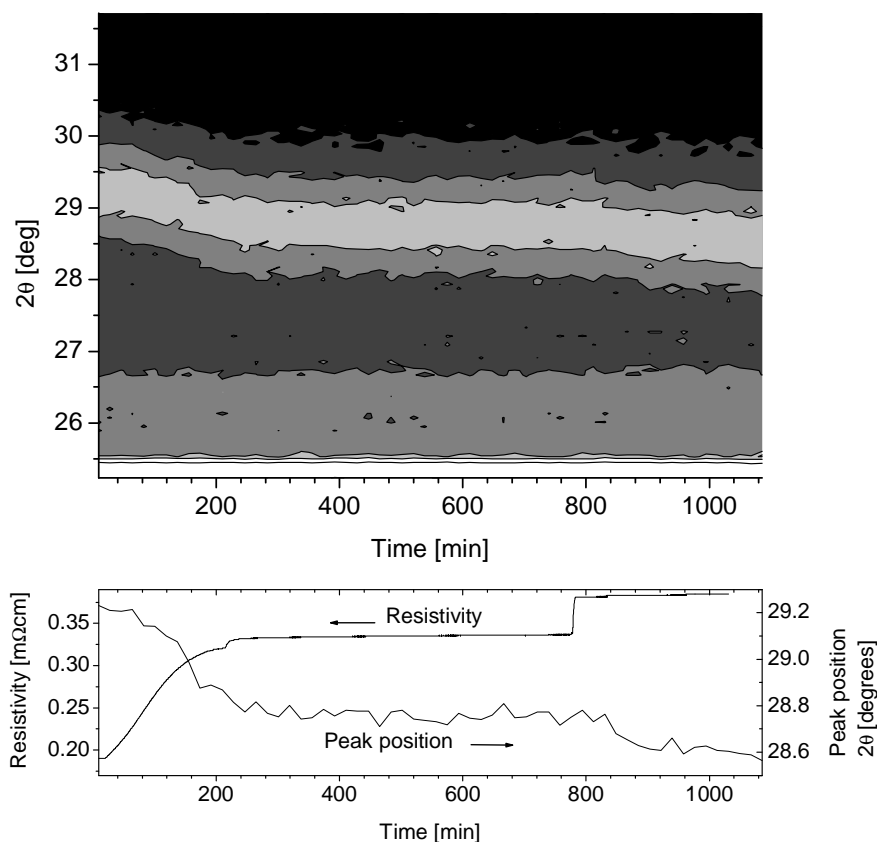
Figure 2.10: During loading of a nanocrystalline \text{YH}_2 film with hydrogen up to 1 bar the Bragg-peak shifts to lower angles indicating a lattice expansion due to hydrogen incorporation. The fcc to hcp phase transition is suppressed for nanocrystalline materials.
