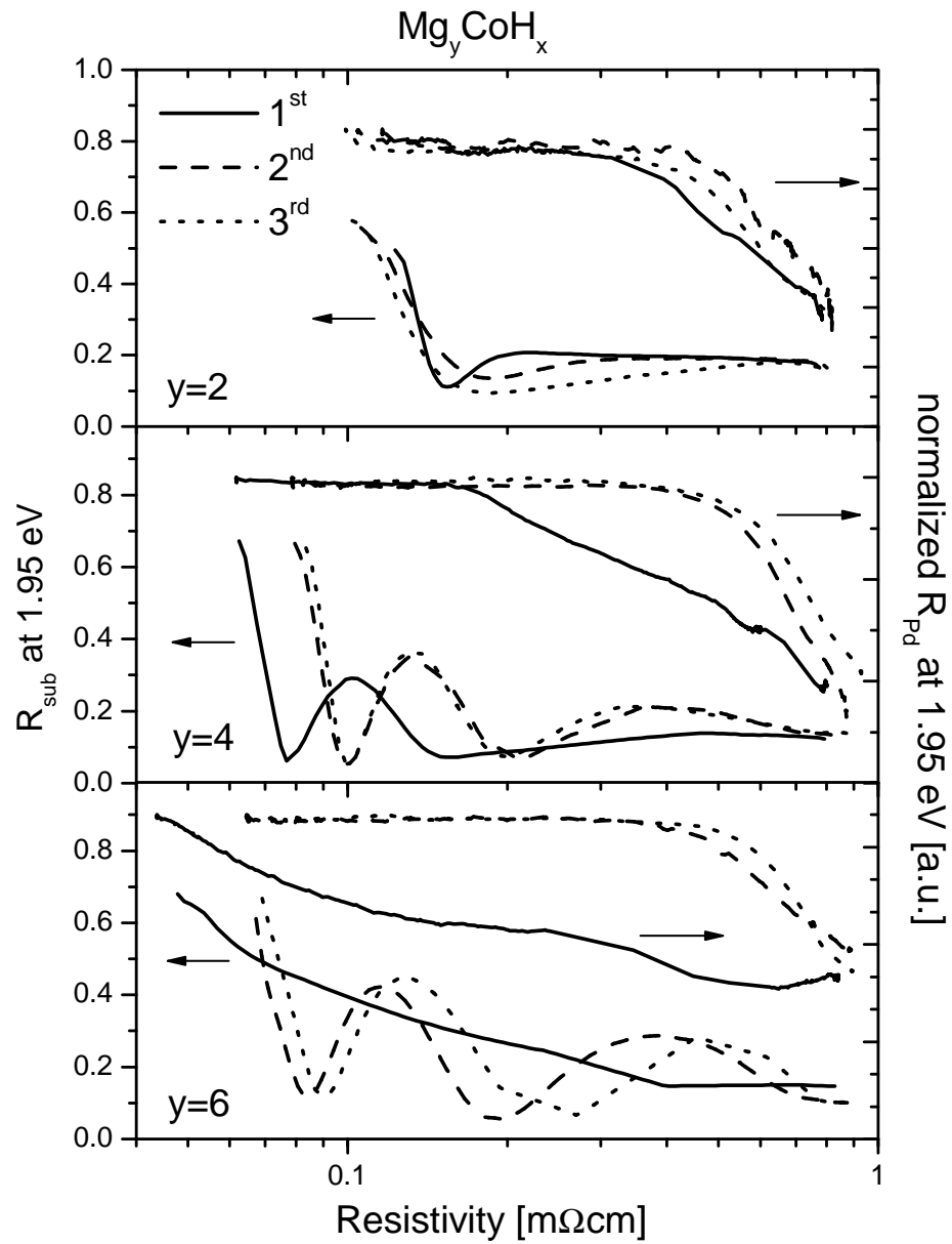
Figure 3.15: Reflection from the Pd top side R_{Pd} and through the transparent substrate R_{sub} at \hbar\omega = 1.95 eV of Mg_yCoH_x with y = 2, 4, 6 for the first few hydrogenation cycles. All R_{Pd} are normalized to the starting value of each hydrogen loading cycle. The 200 nm Mg_yCo films are capped with 10 nm Pd.
