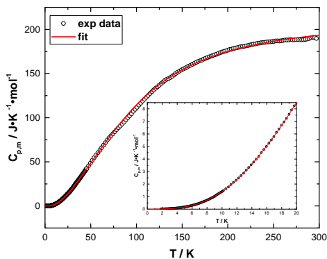
(a) C_{p,m}
