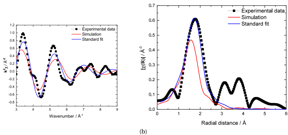
Figure 4.7: (a) Experimental (■) and calculated (red), and fitted (blue) k^2\chi(k) oscillations of (\text{NaF}:\text{ThF}_4) = (0.33:0.67) (absorption, T = 1252 \text{ K} ). (b) Fourier transform modulus |\chi(R)| of the EXAFS spectra.
