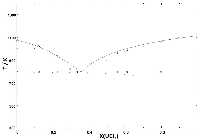
Figure 7.4: NaCl- \text{UCl}_3 phase diagram as calculated in this work, compared to experimental data by Sooby et al. [77] ( \bullet ) and Kraus [47] ( \square ).
