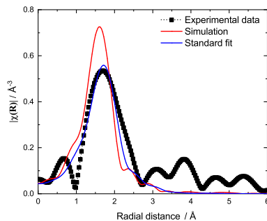
Figure 4.9: (a) Experimental (■), simulated (red), and fitted (blue) k^2\chi(k) oscillations of (KF:ThF 4 ) = (0.67:0.33) (fluorescence, T= 1123 K). (b) Fourier transform modulus |\chi(R)| of the EXAFS spectra.
