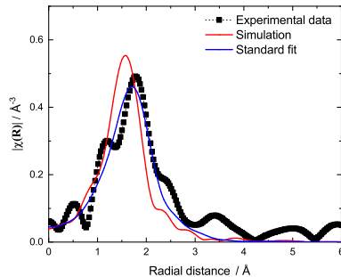
Figure 4.24: (a) Experimental (■), simulated (red), and fitted (blue) k^2\chi(k) oscillations of (\text{KF}:\text{ThF}_4) = (0.50:0.50) (fluorescence, T=1209 K). (b) Fourier transform modulus |\chi(R)| of the EXAFS spectra.
