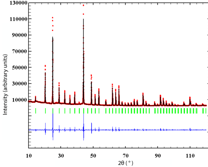
Figure 6.7: Comparison between the observed Y_{obs} (red) and calculated Y_{calc} (black) X-ray diffraction pattern of \beta -Na 2 ThF 6 . Y_{obs} - Y_{calc} (blue) is the difference between the experimental and calculated intensities. The Bragg reflections' angular positions are marked in green. Measurement at \lambda = \text{Cu} - \text{K}\alpha .
