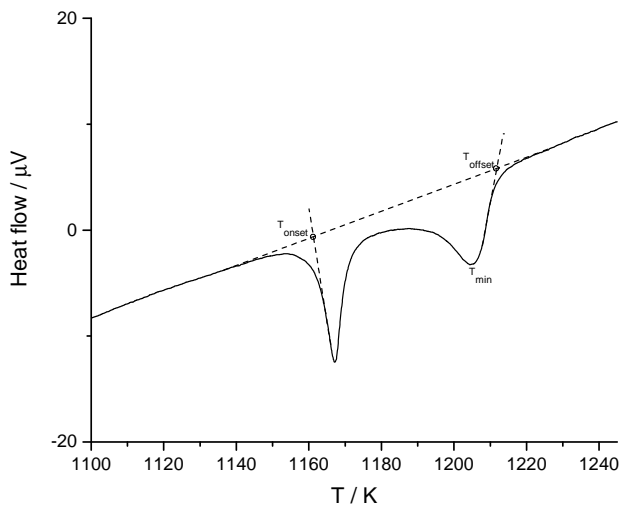
Figure A.3: Representative example of a DSC heating ramp indicating how T_{onset} and T_{offset} were determined. T_{min} was chosen as the liquidus temperature.
