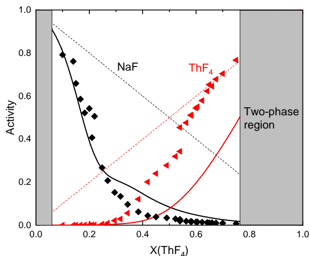
Figure 6.14: Activities in the Na x Th 1-x F 4-3x liquid solution at T = 1241 K. The solid lines correspond to the activities predicted by the present structural-thermodynamic model. The symbols are experimental data by Sidorov et al. [69] at T = 1241 K. The dashed lines represent ideal behavior.
