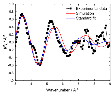
Figure 4.22: (a) Experimental (■), simulated (red), and fitted (blue) k^2\chi(k) oscillations of (\text{NaF}:\text{UF}_4) = (0.50:0.50) (absorption, T = 1033 K). (b) Fourier transform modulus |\chi(R)| of the EXAFS spectra.
