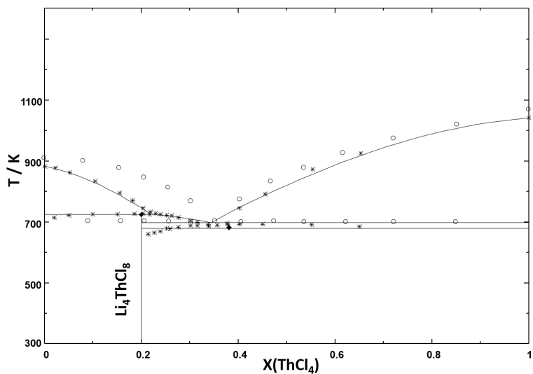
Figure A.1: The \text{LiCl}-\text{ThCl}_4 phase diagram as re-calculated in this work. Symbols: phase diagram data reported by Tanii [58] (*), Oyamada [43] (o), and Vokhmyakov et al. [61] (◆).
