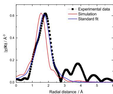
Figure 4.10: (a) Experimental (■), simulated (red), and fitted (blue) k^2\chi(k) oscillations of (KF:UF 4 ) = (0.50:0.50) (absorption, T= 1098 K). (b) Fourier transform modulus |\chi(R)| of the EXAFS spectra.
