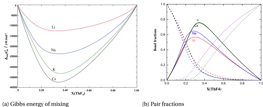
Figure 2.10: (a) Gibbs energy of mixing at T = 1400 K. Red: LiF-ThF 4 , blue: NaF-ThF 4 , green: KF-ThF 4 , black: CsF-ThF 4 . Initial states were the liquid end-members, the final state was the liquid solution. (b) Bond fractions of the LiF-ThF 4 (red) [12], NaF-ThF 4 (blue) [13], KF-ThF 4 (green, this work) and CsF-ThF 4 (black) [48] systems calculated at T = 1400 K. Dashed lines: M-M-F, solid lines: M-Th-F, dotted lines: Th-Th-F-F pair fractions.
