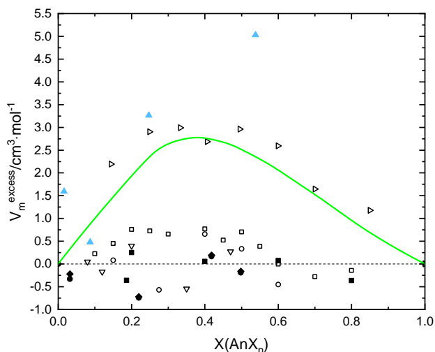
Figure 7.9: Excess molar volumes of the binary mixtures: LiF-UF 4 at T = 1073 K, LiF-ThF 4 at T = 1273 K, NaCl-UF 3 at T = 1020 K. Ideal behavior (dotted line), is calculated using the molar volumes of the end-members from the corresponding study, estimated from linear fits when not available. Green solid line: NaCl-UF 3 , this work. LiF-UF 4 : Klimenkov et al. [45] □, Brown and Porter [11] ○, Blanke et al. [9] ▽; LiF-ThF 4 : Hill et al. [39] ■, Brown and Porter [11] ◆, Porter and Meaker [68] ●; NaCl-UF 3 : Desyatnik et al. [26] ▷, Mochinaga et al. [56] ▲.
