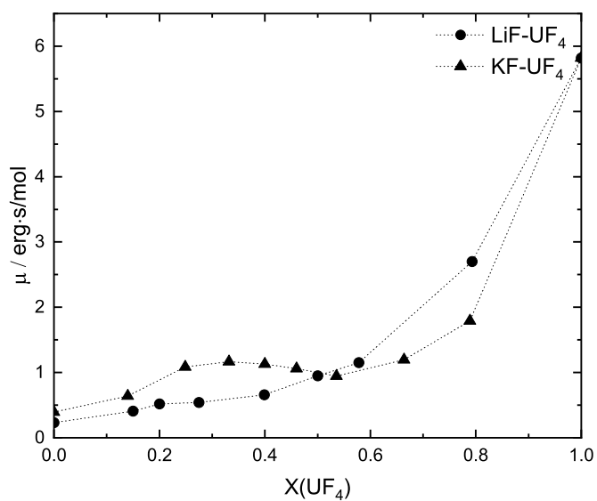
Figure 4.17: Molar viscosity (erg·s/mol) of \text{AF-UF}_4 ( \text{A} = \text{Li}, \text{K} ) melts at an isotherm of T = 1230 \text{ K} . Adapted from [13].
