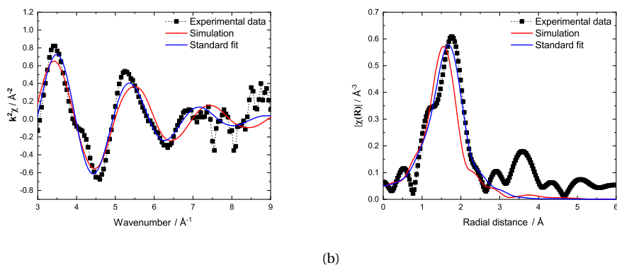
Figure 4.8: (a) Experimental (■) and calculated (red), and fitted (blue) k^2\chi(k) oscillations of (\text{NaF}:\text{UF}_4) = (0.33:0.67) (absorption, T = 1153 \text{ K} ). (b) Fourier transform modulus |\chi(R)| of the EXAFS spectra.
