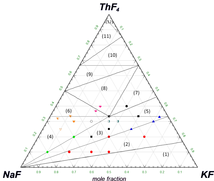
Figure 2.15: Projection of the \text{NaF-KF-ThF}_4 ternary system as calculated in this study at 300 K superimposed against experimental compositions analyzed using XRD by [16]; red circles: \{\text{NaF} + \text{K}_3\text{ThF}_7 + \text{KF}\} ; blue triangles: \{\text{NaF} + \text{K}_3\text{Th}_2\text{F}_{11} + \text{K}_3\text{ThF}_7\} ; black squares: unidentified patterns; green diamonds: \{\text{NaF} + \text{KNaThF}_6\} ; half-filled squares: phase similar to \text{KNaThF}_6 and unidentified lines; half-filled circle: \{\text{KNaThF}_6\} ; black circle: \{\text{KNaThF}_6 + \text{KThF}_5\} ; half-filled diamond: \{\text{KThF}_5 + \text{KNaThF}_6 + \text{unidentified lines}\} ; half-filled orange triangle: \{\text{Na}_2\text{ThF}_6 + \text{unidentified lines}\} ; filled orange triangle: \{\text{Na}_2\text{ThF}_6 + \text{KNaThF}_6\} ; empty orange triangle: \{\text{Na}_2\text{ThF}_6 + \text{KNaThF}_6 + \text{Na}_4\text{ThF}_8(?)\} ; white circle: \{\text{KNaThF}_6 + \text{weak lines}\} . These data are also compared in Table 2.13 for more clarity. Phases in equilibrium in phase fields (1)-(11) are listed in section 2.5.7.
