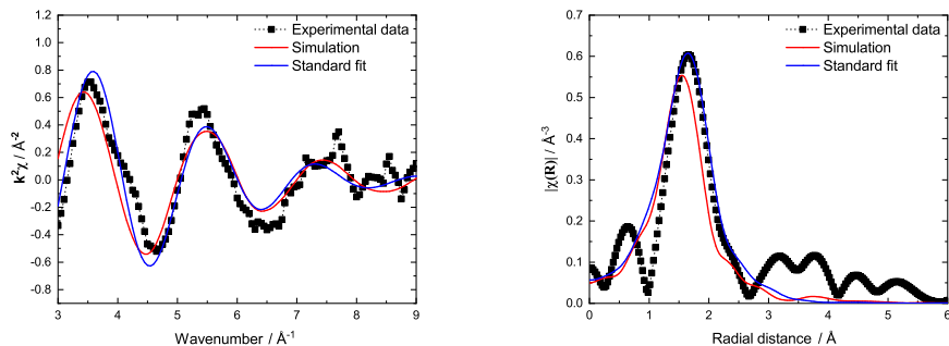
Figure 4.26: (a) Experimental (■), simulated (red), and fitted (blue) k^2\chi(k) oscillations of (\text{KF}:\text{UF}_4) = (0.33:0.67) (absorption, T= 1090 K). (b) Fourier transform modulus |\chi(R)| of the EXAFS spectra.
