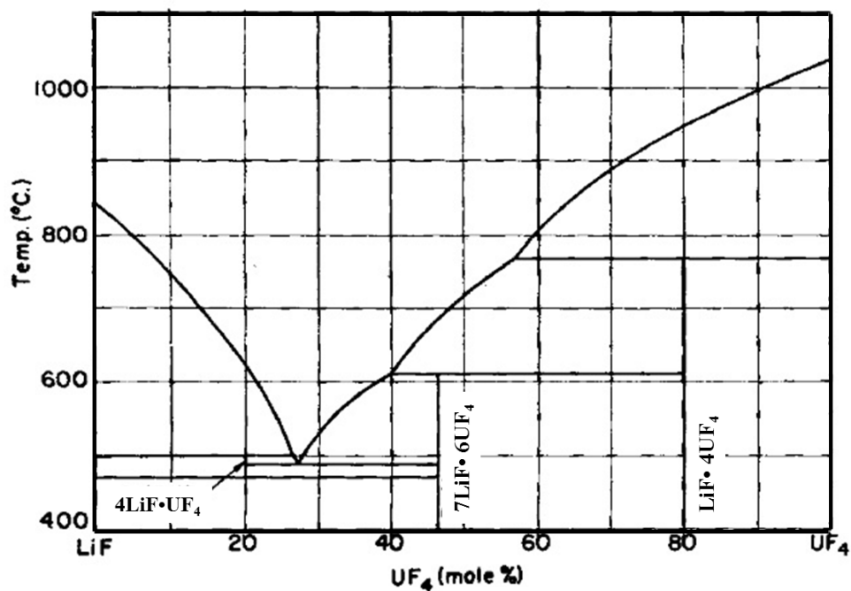
Figure 5.1: The system \text{LiF-UF}_4 as reported by Barton et al.[4]. Reproduced with permission from Wiley and Sons.
