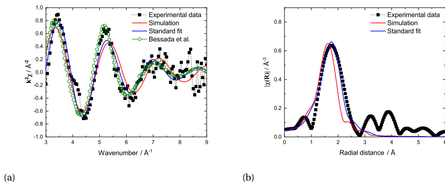
Figure 4.6: (a) Experimental (■, [46]), simulated (red), and fitted (blue) k^2\chi(k) oscillations of (\text{LiF}:\text{ThF}_4) = (0.75:0.25) (fluorescence, T = 898 K). Dotted green line: experimental data by Bessada et al. [5] at the same composition (absorption, T = 973 K). (b) Fourier transform modulus |\chi(R)| of the EXAFS spectra.
