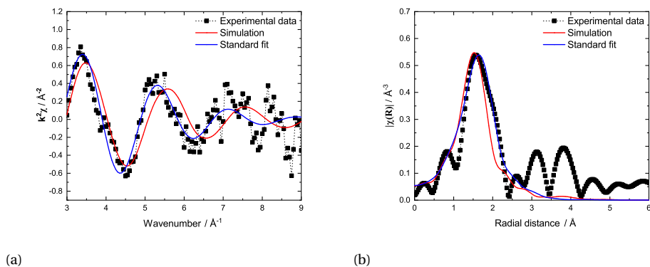
Figure 4.28: (a) Experimental (■), simulated (red), and fitted (blue) k^2\chi(k) oscillations of (\text{CsF}:\text{UF}_4) = (0.33:0.67) (fluorescence, T= 1191 K). (b) Fourier transform modulus |\chi(R)| of the EXAFS spectra.
