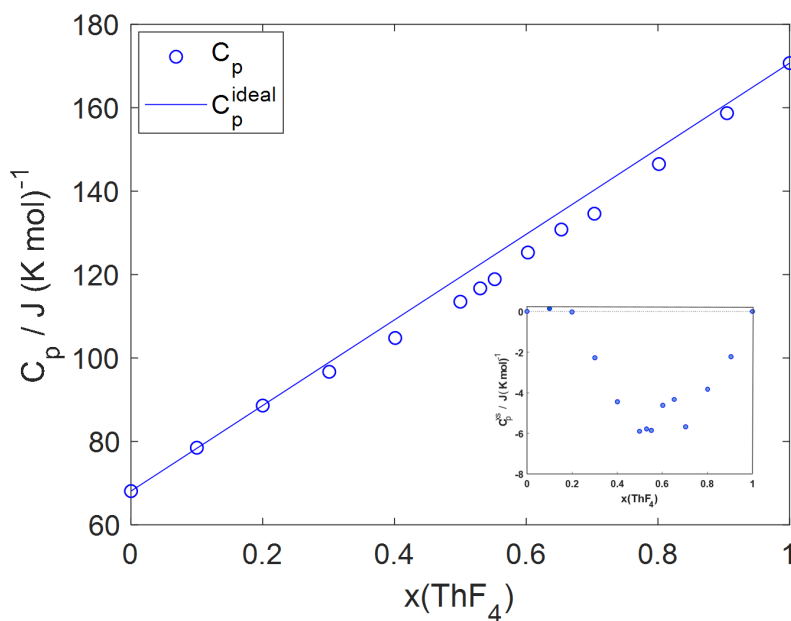
Figure 6.11: Evolution of heat capacity and ideal heat capacity in the NaF- \text{ThF}_4 system calculated from enthalpies obtained in MD simulations in the temperature region 1433 - 2000 K. Inset: excess heat capacity.
