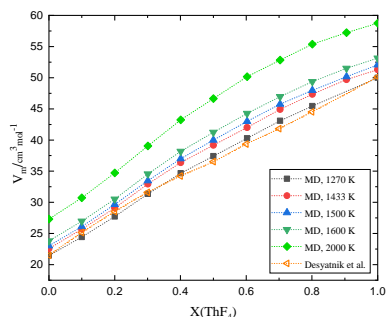
Figure 6.1: (a) Molar volumes versus composition at T = 1270, 1433, 1500, 1600 , and 2000 K. (b) Excess molar volumes versus composition at the same temperatures. Both are compared to data by Desyatnik et al.[18] at 1270 K.
