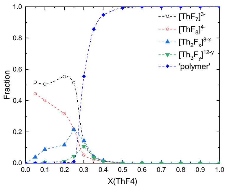
Figure 6.5: Fraction of monomers ( \circ ), dimers ( \diamond ), and 'polymers' ( \blacktriangle ), in the NaF-ThF 4 liquid solution at T = 1433 K.
