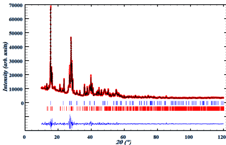
Figure 2.1: Diffractogram of the K 5 ThF 9 -K 2 ThF 6 mixture X(\text{ThF}_4) = 0.17 . Comparison between the observed ( Y_{obs} , in red) and calculated ( Y_{calc} , in black) X-ray diffraction patterns. Y_{obs} - Y_{calc} , in blue, is the difference between the experimental and calculated intensities. The Bragg's reflection angular positions are marked in blue (K 2 ThF 6 ), and red (K 5 ThF 9 ).
