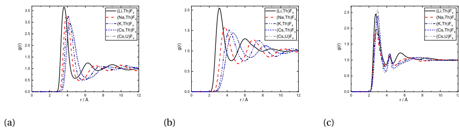
Figure 4.30: Radial distribution functions: (a) An-A, (b) A-A, and (c) F-F in the AF- \text{AnF}_4 melts at composition X(\text{AnF}_4) = 0.25 (Li and Cs-based melts) and X(\text{AnF}_4) = 0.33 (Na and K-based melts).
