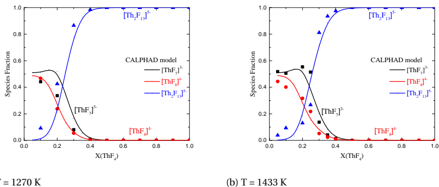
Figure 6.13: Complex anion distribution obtained with the CALPHAD model (solid lines) and compared with the MD data shown in Fig. 6.19 (symbols): [ThF 7 ] 3- (black), [ThF 8 ] 4- (red), and [Th 2 F 13 ] 5- (blue). (a) T = 1270 K, (b) T = 1433 K.
