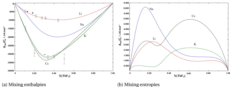
Figure 2.9: (a) Mixing enthalpies and (b) mixing entropies of the LiF-ThF 4 (red) [12], NaF-ThF 4 (blue) [13], KF-ThF 4 (green, this work) and CsF-ThF 4 (black) [48]. The calculations were done at T = 1400 K considering KF(l) and ThF 4 (l) as initial states and the liquid solution as the final state.
