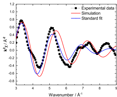
Figure 4.25: (a) Experimental (■), simulated (red), and fitted (blue) k^2\chi(k) oscillations of (\text{KF}:\text{ThF}_4) = (0.33:0.67) (absorption, T=1266 K). (b) Fourier transform modulus |\chi(R)| of the EXAFS spectra.
