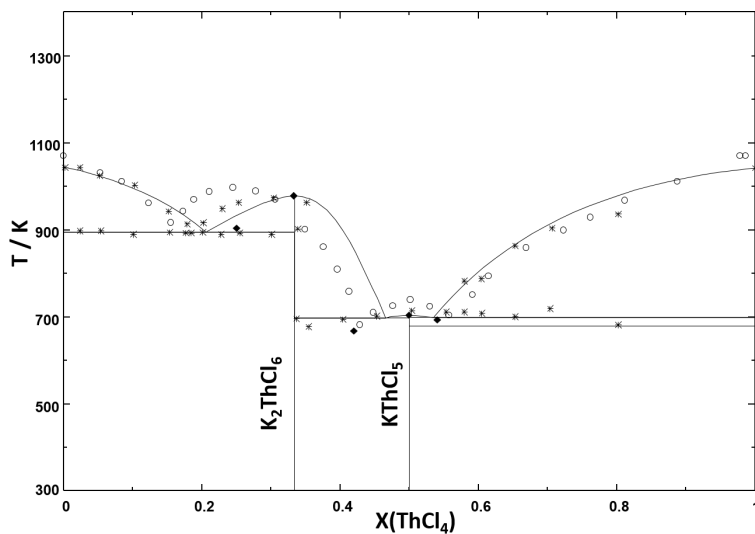
Figure A.3: The \text{KCl-ThCl}_4 phase diagram as re-calculated in this work. Symbols: phase diagram data reported by Tanii [58] (*), Oyamada [43] ( \circ ), and Vokhmyakov et al. [61] ( \blacklozenge ).
