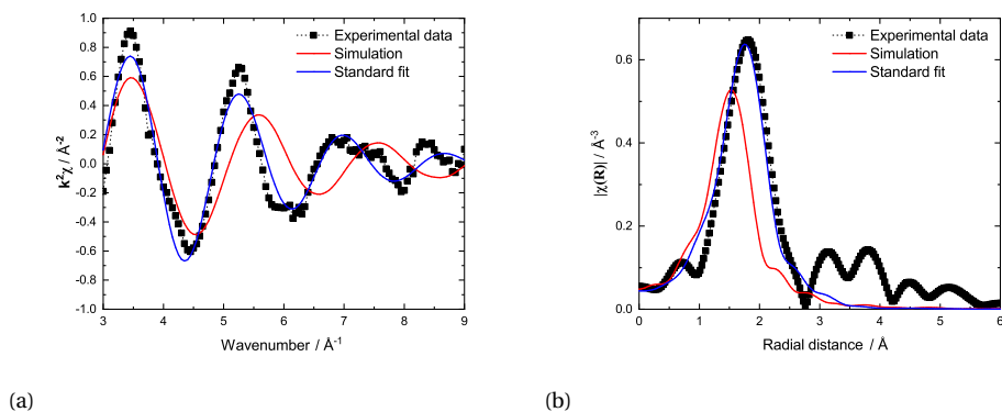
Figure 4.29: (a) Experimental (■), simulated (red), and fitted (blue) k^2\chi(k) oscillations of (\text{CsF}:\text{ThF}_4) = (0.50:0.50) (absorption, T= 1201 K). (b) Fourier transform modulus |\chi(R)| of the EXAFS spectra.
