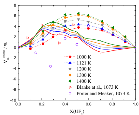
Figure 5.11: Evolution of density. (a) Solid lines: isotherms calculated from the empirical equations reported by Klimenkov et al. [44]; solid symbols: results derived from MD simulations; \triangleright , red, experimental data by Blanke et al. [9] and \circ (purple) by Porter and Meaker [64], T = 1073 K. (b) Relative excess molar volume (%), of the (Li,UF) x solution.
