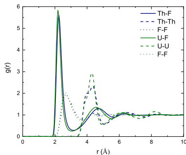
Figure 4.3: Pairwise radial distribution functions of molten UF 4 and ThF 4 calculated with MD at T = 1357 K and T = 1433 K, respectively.
