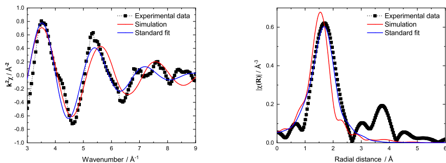
Figure 4.27: (a) Experimental (■), simulated (red), and fitted (blue) k^2\chi(k) oscillations of (\text{CsF}:\text{UF}_4) = (0.50:0.50) (absorption, T= 1058 K). (b) Fourier transform modulus |\chi(R)| of the EXAFS spectra.
