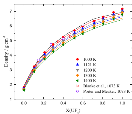
Figure 5.11: Evolution of density. (a) Solid lines: isotherms calculated from the empirical equations reported by Klimenkov et al. [44]; solid symbols: results derived from MD simulations; \triangleright , red, experimental data by Blanke et al. [9] and \circ (purple) by Porter and Meaker [64], T = 1073 K. (b) Relative excess molar volume (%), of the (Li,UF) x solution.
