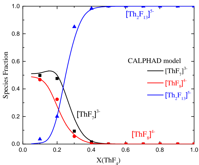
Figure 6.20: Distribution of the 7, 8 and 9 coordinated [\text{ThF}_n]^{m-} complexes versus composition in the NaF-ThF 4 system at 1320 K.
