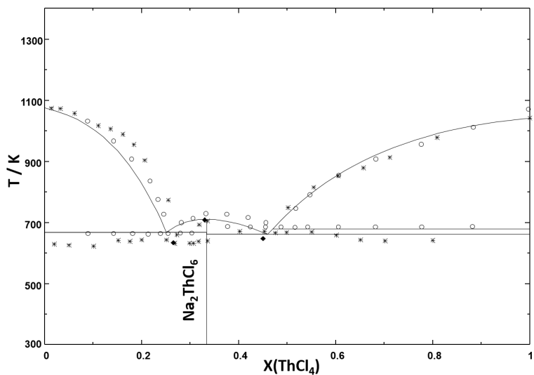
Figure A.2: The \text{NaCl}-\text{ThCl}_4 phase diagram as re-calculated in this work. Symbols: phase diagram data reported by Tanii [58] (*), Oyamada [43] (o), and Vokhmyakov et al. [61] (◆).
