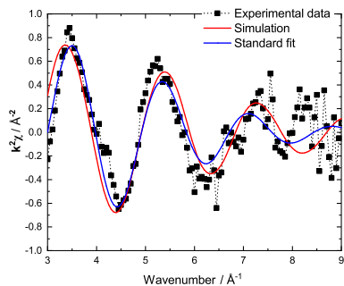
Figure 4.23: (a) Experimental (■), simulated (red), and fitted (blue) k^2\chi(k) oscillations of (\text{KF}:\text{ThF}_4) = (0.833:0.167) (fluorescence, T = 1060 K). (b) Fourier transform modulus |\chi(R)| of the EXAFS spectra.
