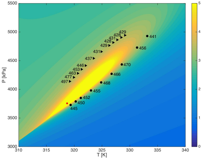
Figure 3.7: Prandtl number values (color coding) of SF 6 as a function of temperature and pressure at supercritical conditions. Red dot: Supercritical point of SF 6 , black triangles: mean temperature and pressure of the experimental data of the upper branch of the iso-Prandtl curve, black circles: mean temperature and pressure of the experimental data of the lower branch of the iso-Prandtl curve. Each data point is labeled with the value of its Nusselt number. The data points are chosen on a Pr_{NOB} = 3.5 isoline. The fluid properties were taken from the NIST database, version 9.1 [25].
