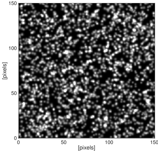
Figure 5.5: Example of computer generated background dot pattern for BOS measurements. This kind of background was made 2000 \times 2000 pixels with a mean diameter of the white dots of about 2 pixels, and it was printed with dimensions of 80 \times 80 mm 2 .
