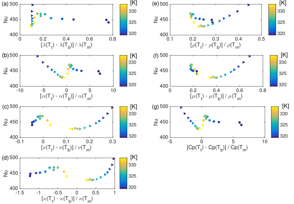
Figure 3.9: Nusselt number as a function of the temperature dependency of the fluid properties of \text{SF}_6 , expressed as the difference between the top and the bottom value of the property over the property value at the average bottom-top temperature ( T_m ). (a), \lambda : thermal conductivity; (b), \alpha : volumetric thermal expansion coefficient; (c), \nu : kinematic viscosity; (d), \kappa : thermal diffusivity; (e), \rho : density; (f), \mu : dynamic viscosity; (g), C_p : specific heat capacity. In all the panels the data are represented by triangles or circles as introduced in Figure 3.7, with color representing their temperature. All the data points are at Pr = 3.5 and Ra_{NOB} = 2.8 \times 10^{11} . The fluid properties were taken from the Coolprop database [31].
