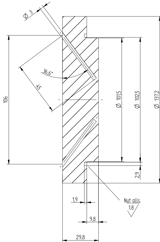
Figure 3.4: Vertical cross-section ( 90^\circ rotated in clockwise direction) of the bottom copper plate of the cell. From the section the two holes for the thermocouples are visible.
