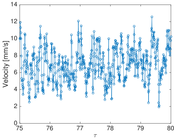
Figure 5.30: Zoom-in of Figure 5.29 for 75 < \tau < 80 . Velocity in a rectangular region of 10 \times 15 data points centered in X/H \approx 0.9 and Y/H \approx 0.5 over the number of turnover times \tau for the experiment SC_{gas} ( Ra_{NOB} = 5.33 \times 10^{11} , Pr = 4.15 ).
