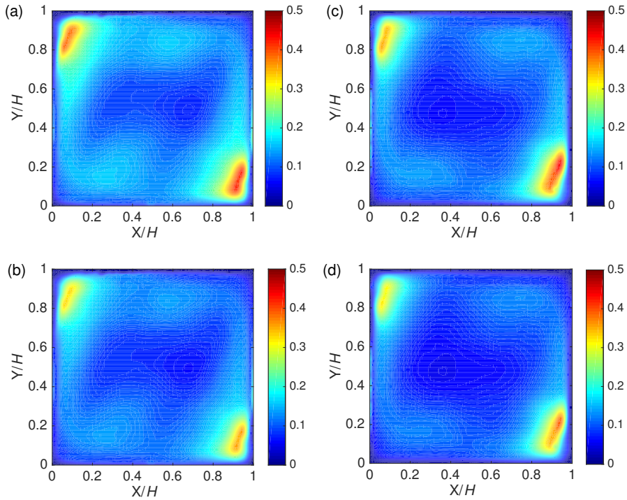
Figure 2.7: Turbulent kinetic energy in a vertical cross section at half-depth of the cell ( Z/H = 0.5 ) (repeated experiments). Values normalized by U_{LSC(GL)} in panels (a) and (c) and by U_{LSC(P)} in panels (b) and (d). Panels (a) and (b), Non-Oberbeck-Boussinesq 2^{nd} : Ra_{NOB} = 6.84 \times 10^8 , Pr_{NOB} = 4.33 ; panels (c) and (d), Oberbeck-Boussinesq 2^{nd} : Ra_{NOB} = 6.77 \times 10^8 , Pr_{NOB} = 7.24 .
