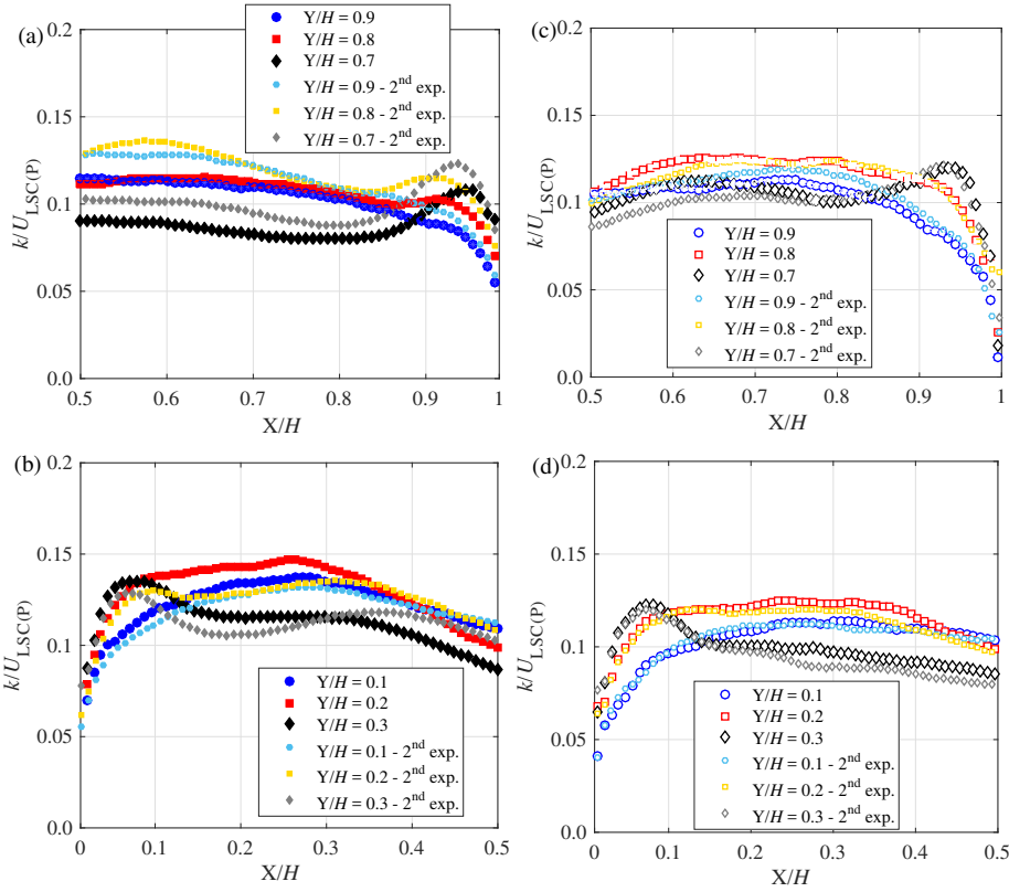
Figure 2.9: One-line plots of the turbulent kinetic energy values at several heights Y/H ( Y/H = 0.1, 0.2, 0.3, 0.7, 0.8, 0.9 ) along the axis X/H at Z/H = 0.5 . Values normalized by U_{LSC(P)} . a), b), Non-Oberbeck-Boussinesq: Ra_{NOB} = 6.9 \times 10^8 , Pr_{NOB} = 4.33 , Non-Oberbeck-Boussinesq 2 nd : Ra_{NOB} = 6.84 \times 10^8 , Pr_{NOB} = 4.33 . c), d), Oberbeck-Boussinesq: Ra_{NOB} = 6.7 \times 10^8 , Pr_{NOB} = 7.24 , Oberbeck-Boussinesq 2 nd : Ra_{NOB} = 6.77 \times 10^8 , Pr_{NOB} = 7.24 .
