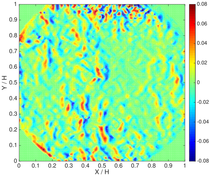
Figure 5.18: (a) Instantaneous BOS image displacement of the experiment SC_{max\Delta\rho} , after subtraction of the time average image displacement of that experiment (shown in Figure 5.15). (b) Magnitude of the spatial gradient ( \nabla d ) of the BOS image displacement shown in panel (a).
