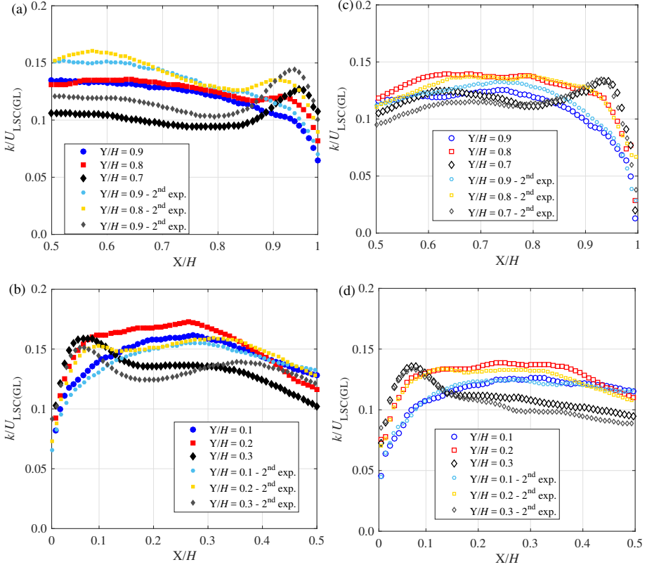
Figure 2.8: One-line plots of the turbulent kinetic energy values at several heights Y/H ( Y/H = 0.1, 0.2, 0.3, 0.7, 0.8, 0.9 ) along the axis X/H at Z/H = 0.5 . Values normalized by U_{LSC(GL)} . a), b), Non-Oberbeck-Boussinesq: Ra_{NOB} = 6.9 \times 10^8 , Pr_{NOB} = 4.33 , Non-Oberbeck-Boussinesq 2^{nd} : Ra_{NOB} = 6.84 \times 10^8 , Pr_{NOB} = 4.33 . c), d), Oberbeck-Boussinesq: Ra_{NOB} = 6.7 \times 10^8 , Pr_{NOB} = 7.24 , Oberbeck-Boussinesq 2^{nd} : Ra_{NOB} = 6.77 \times 10^8 , Pr_{NOB} = 7.24 .
