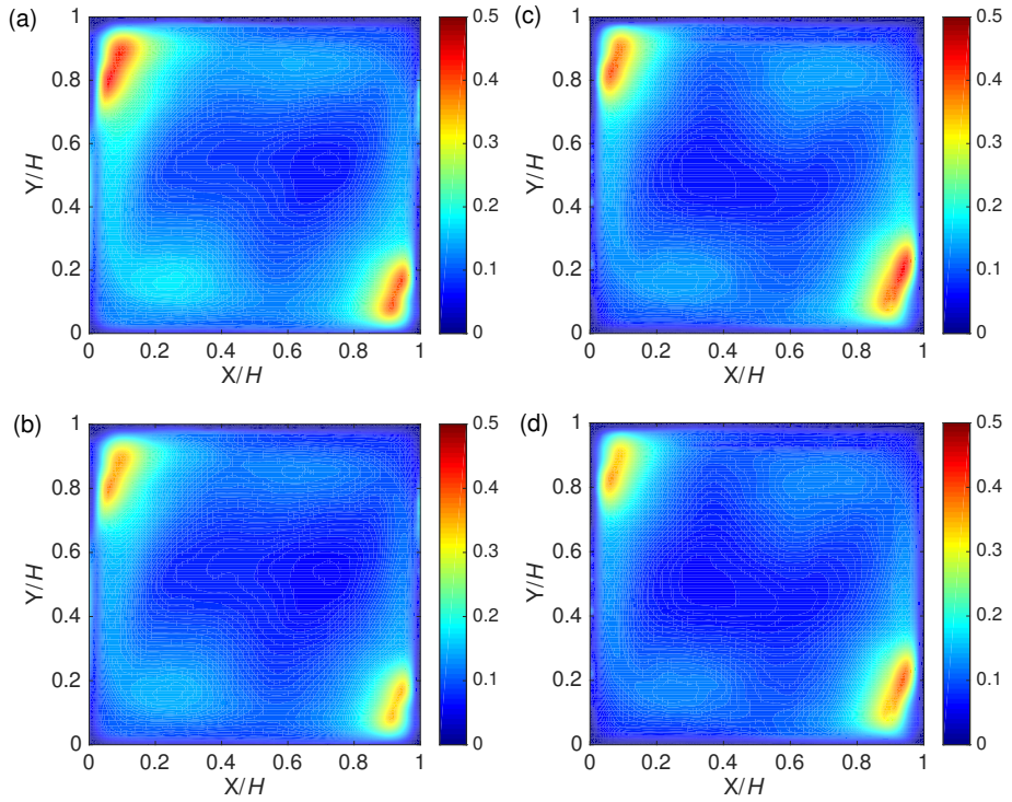
Figure 2.6: Turbulent kinetic energy in a vertical cross section at half-depth of the cell ( Z/H = 0.5 ). Values normalized by U_{LSC}^{(GL)} in panels (a) and (c) and by U_{LSC}^{(P)} in panels (b) and (d). Panels (a) and (b), Non-Oberbeck-Boussinesq: Ra_{NOB} = 6.91 \times 10^8 , Pr_{NOB} = 4.33 ; panels (c) and (d), Oberbeck-Boussinesq: Ra_{NOB} = 6.74 \times 10^8 , Pr_{NOB} = 7.24 .
