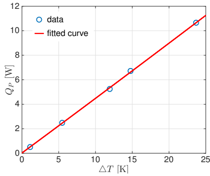
Figure 3.5: Parasite heat losses ( Q_p ) through the lateral walls of the cell and the external insulation material, as a function of the difference of temperature between the plates ( \Delta T ), when the cell is under vacuum. Empty circles represent the measured data and the red line is their fitting curve.
