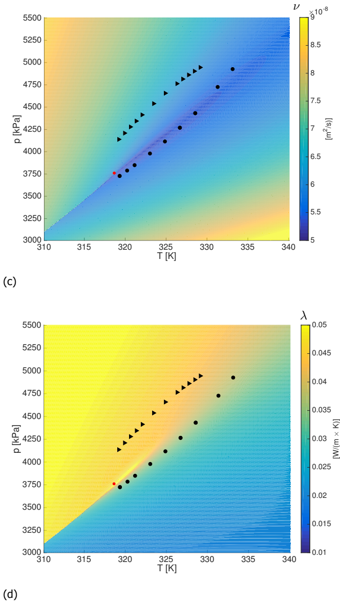
Figure 3.10: (a) Specific heat capacity of SF_6 , C_p as a function of temperature and pressure; (b) Isobaric thermal expansion coefficient, \alpha , as a function of temperature and pressure; (c) Kinematic viscosity of SF_6 , \nu , as a function of temperature and pressure; (d) Thermal conductivity of SF_6 , \lambda , as a function of temperature and pressure. Black triangles and circles: experimental data-points. Small red circle: supercritical point of SF_6 . Fluid property values taken from the CoolProp database [31].
