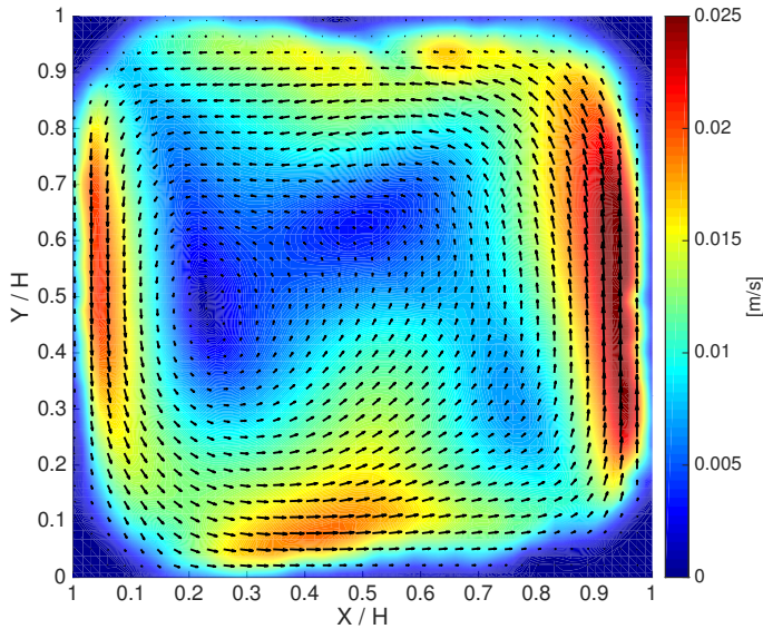
Figure 5.34: Time averaged velocity field of the PIV experiment SC_{liquid}.Ra_{NOB}=5.44 \times 10^{11} , Pr_{NOB} = 4.89 . The color scale indicates the magnitude of the mean velocity \bar{u} , while the arrows show its direction. Only one arrow every four data points is plotted.
