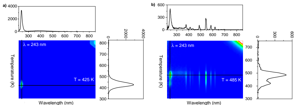
Figure 4.6: TL emission spectrum of a) YPO 4 :1.0% Bi and b) YPO 4 :1.0% Bi, 1.0% Tb recorded after \gamma -ray irradiation for 2 h using a 60 Co source.
