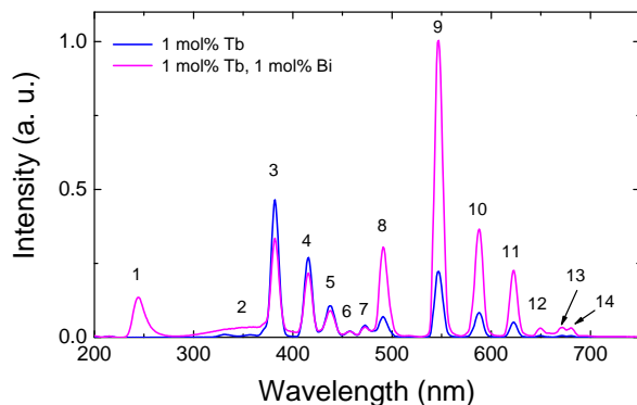
Figure 4.5: X-ray excited emission spectra of YPO 4 :1%Tb 3+ and YPO 4 :1%B 3+ ,1%Tb 3+ measured at room temperature.
