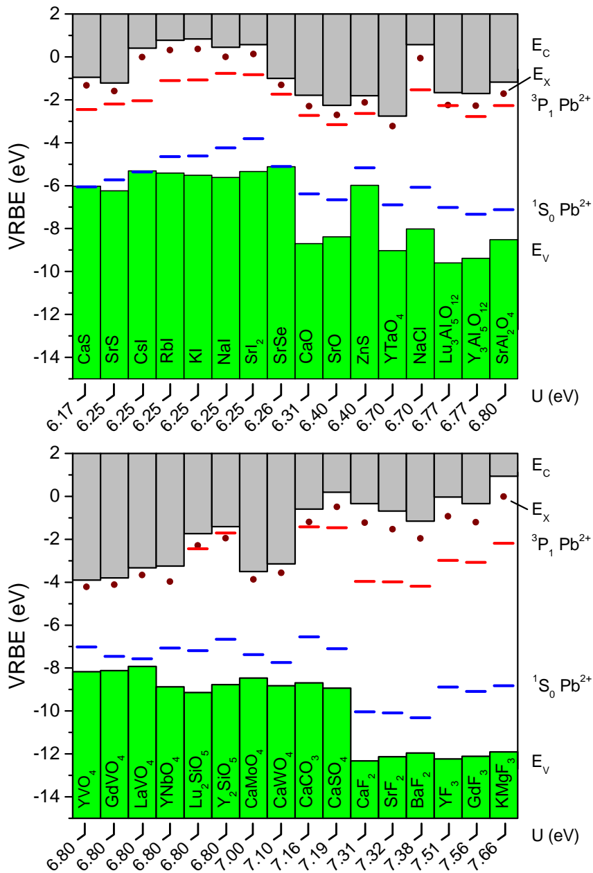
Figure 7.6: Stacked VRBE diagrams for Pb 2+ doped compounds. E C is the binding energy at the conduction band bottom, E X is the binding energy in the host exciton, E V is the binding energy at the valence band top and 1S 0 and 3P 1 are the binding energies in the Pb 2+ ground and excited state, respectively.
