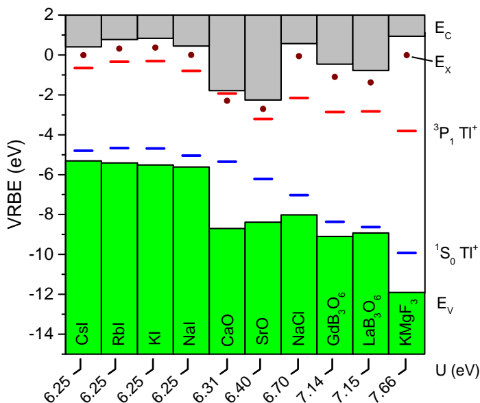
Figure 7.7: Stacked VRBE diagrams for Tl^+ doped compounds. E_C is the binding energy at the conduction band bottom, E_X is the binding energy in the host exciton, E_V is the binding energy at the valence band top and ^1S_0 and ^3P_1 are the binding energies in the Tl^+ ground and excited state, respectively.
