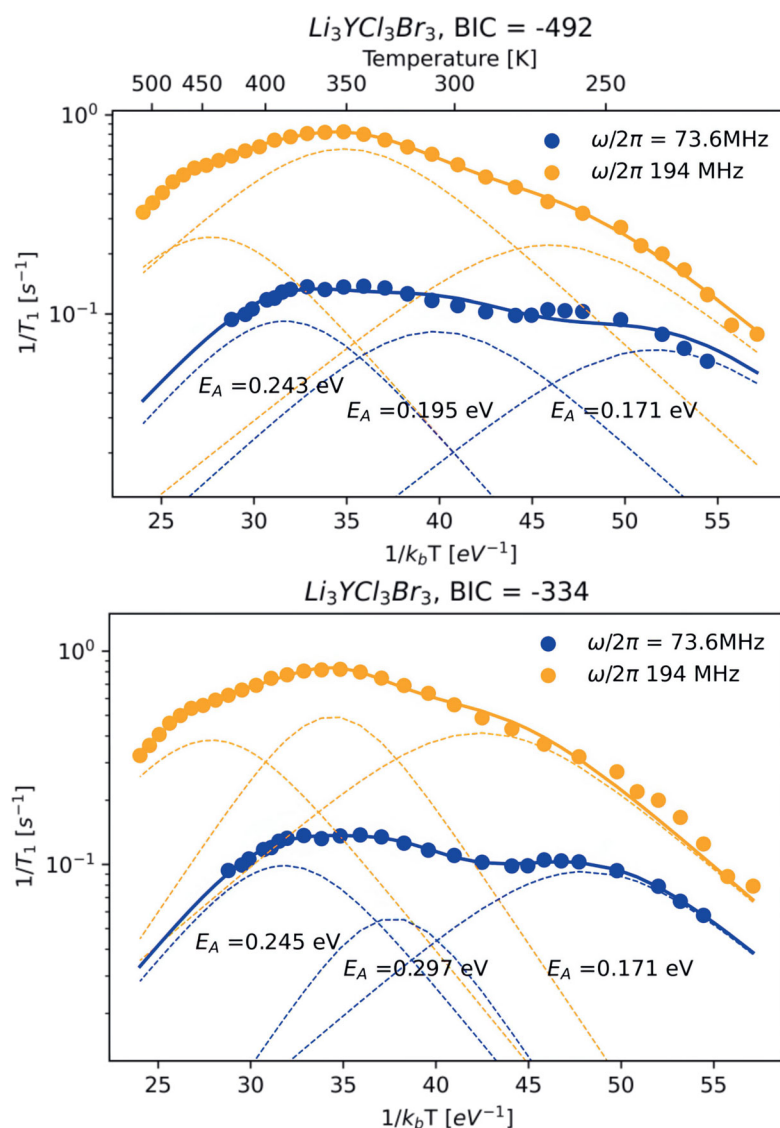
Figure 4.12: Relaxation rates 1/T_1 of {}^6\text{Li} and {}^7\text{Li} of \text{Li}_3\text{YCl}_3\text{Br}_3 fit using a model containing of three independent BPP-type jump processes, once without weighing the residuals (top) and once by weighing the data measured at 73.6MHz by a factor N=4 (bottom). The E_a [eV] of the individual processes are indicated in the plot. BIC stands for Bayesian information criterion, models with lower BIC are usually preferred.
