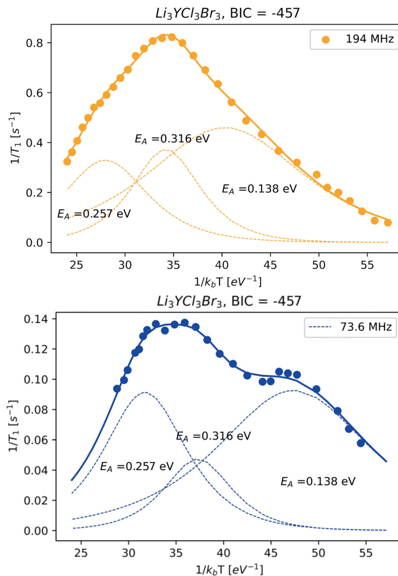
Figure 8.5: Relaxation rates 1/T_1 of {}^7\text{Li} (top) and {}^6\text{Li} (bottom) of \text{Li}_3\text{YCl}_3\text{Br}_3 fit using a model containing of three independent BPP-type jump processes. E_a [eV] of the individual processes are indicated in the plot. The residuals of the two dataset were weighed differently by an additional factor 4 for the dataset measured at 73.6 MHz.
