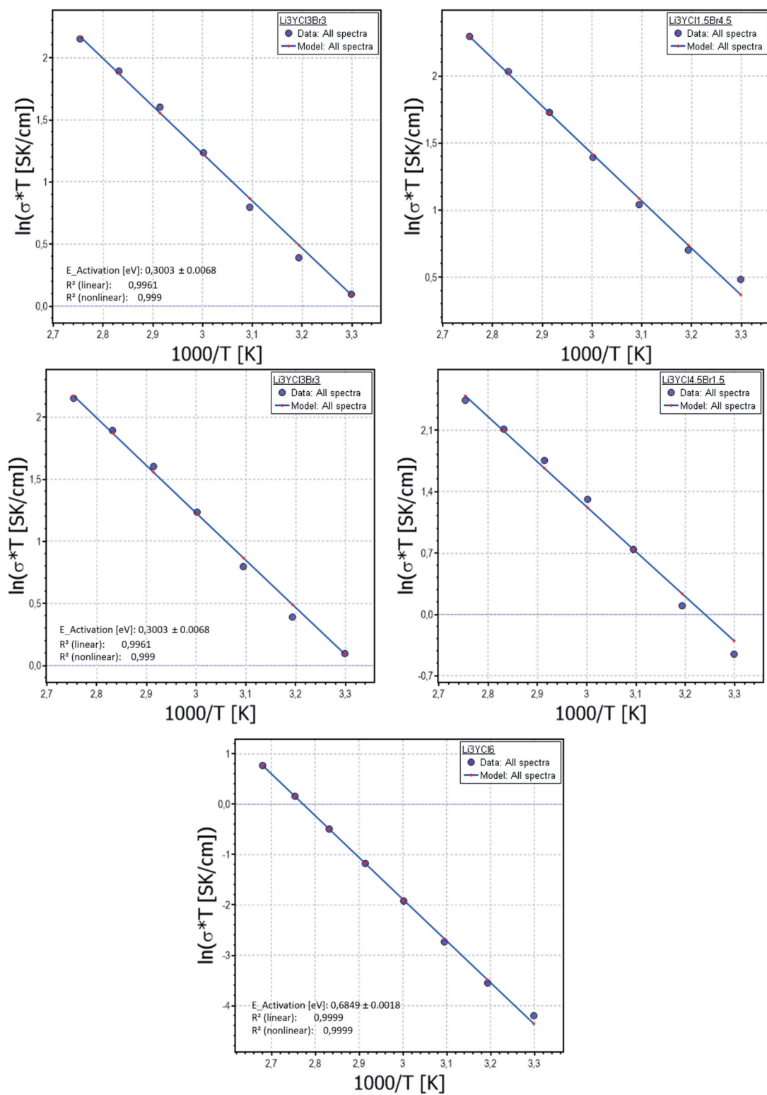
Figure 8.32: Arrhenius relationships of \text{Li}_3\text{YBr}_x\text{Cl}_{6-x}
