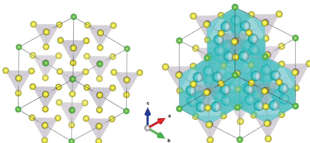
Figure 4.5: Visualization of the crystal structure of \text{Li}_6\text{PS}_5\text{X} as published by Deiseroth et al [13]. On the left, the structure is shown without the lithium sites, to illustrate the close packed nature. Cl is shown in green, S in yellow and the pink tetrahedra belong to the \text{PS}_4^{3-} units. On the right, the same angle is shown including the lithium sites and polyhedra (turquoise). There are three cages shown in the structure, one at the top and two at the bottom, as can be imagined by the three turquoise hexagon. The hexagon share edge.
