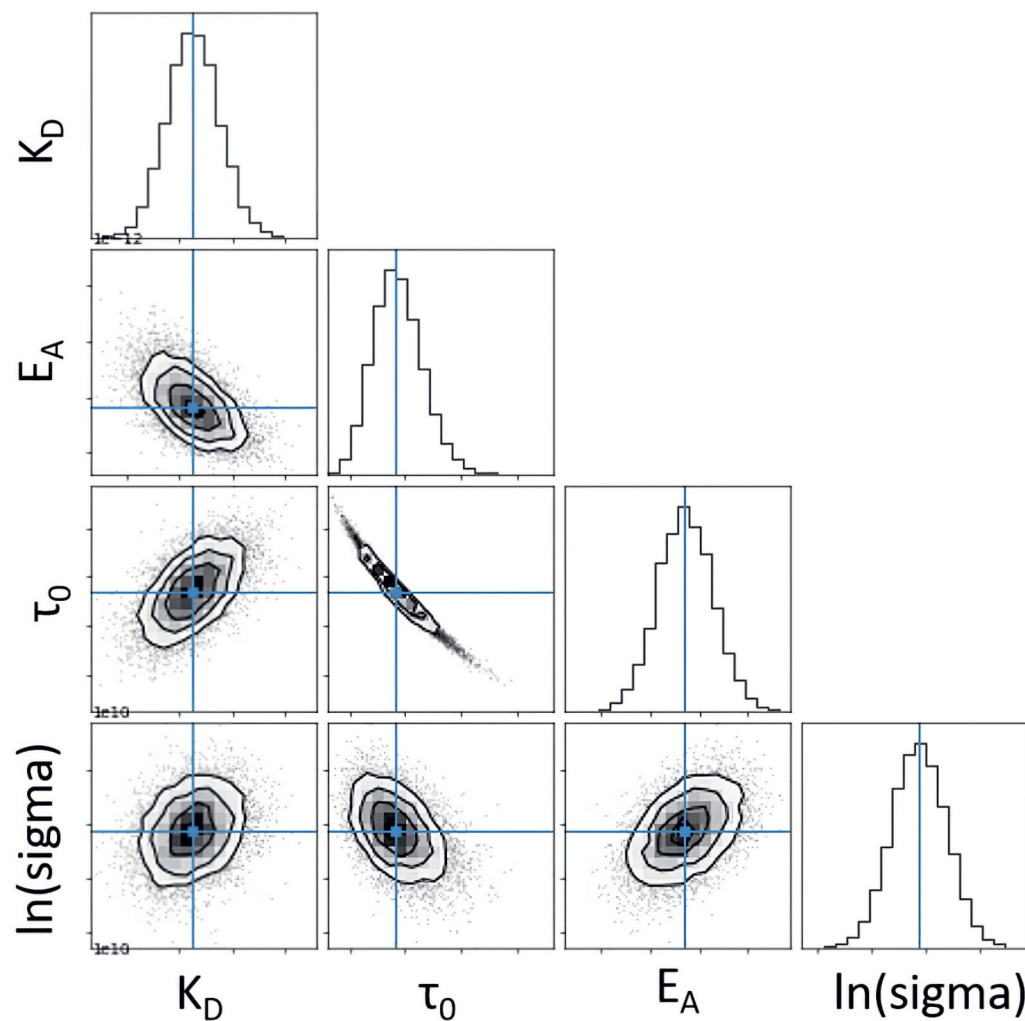
Figure 4.4: Visualization of the a corner plot for a BPP-type fit for the \text{Li}_6\text{PS}_5\text{Cl} used in section 4.2. Both axes (x and y) list the parameter of the fit. The contour plots belonging to two different parameter visualize the relationship between them. The histogram shows the posterior probability distribution of the parameter on the x-axis. The histogram is useful for the decision which parameter estimate is the most appropriate (median, maximum likelihood etc.) and serves to calculate the standard error estimated as half the difference between the 15.8% and 84.2% percentiles. The uncertainty of the data s_n = \exp(\ln\text{sigma}) .
