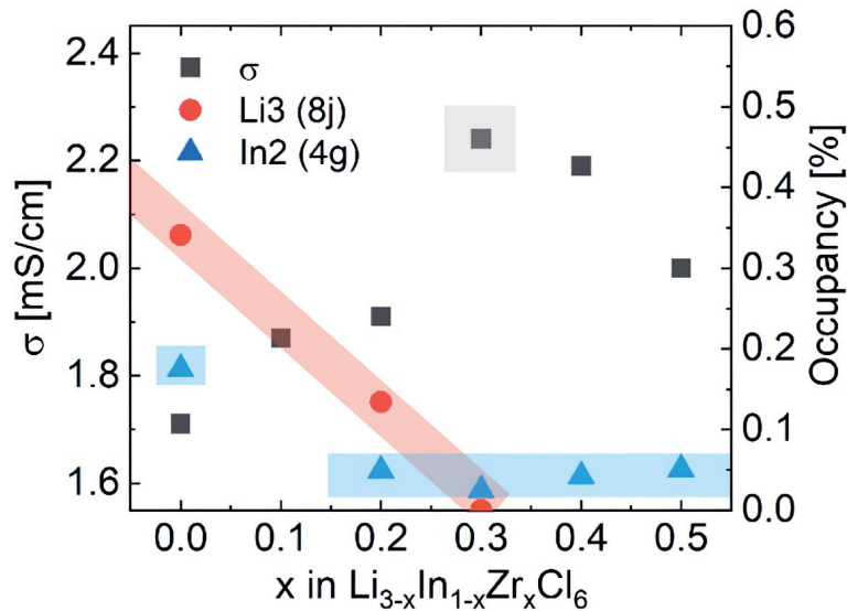
Figure 5.8: Comparison of the ionic conductivity \sigma as measured from impedance with the occupancies of the Li3 (8j) and In2 (4g) sites for \text{Li}_{3-x}\text{In}_{1-x}\text{Zr}_x\text{Cl}_6 . The conductivity reaches its maximum as the tetrahedral Li3 (8j) site disappears. The occupancy of the In2 (4g) site drops to its minimum value already before the maximum in ionic conductivity is reached.
