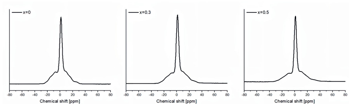
Figure 8.22: {}^7\text{Li} static NMR spectra of \text{Li}_{3-x}\text{In}_{1-x}\text{Zr}_x\text{Cl}_6 , at 9.4T (156 MHz) at T = 493\text{ K} . The central transition is motionally narrowed in all three samples. The shape of the satellites can only be approximated by a combination of quadrupolar coupling as well as chemical shift anisotropy, see Figure S14. The shape is most pronounced in \text{Li}_3\text{InCl}_6 , and slightly flattens for the doped samples. The residual chemical shift anisotropy that resolves at the satellites indicates that the motion of the Li-ions across the different sites does not average out completely.
