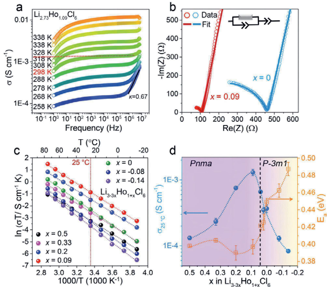
Figure 7.3: a) Conductivity isotherms \sigma(\nu) of the as-prepared \text{Li}_{2.73}\text{Ho}_{1.09}\text{Cl}_6 SSE recorded at different temperatures. b) Representative Nyquist-plots for the as-prepared Pnma phase \text{Li}_{2.73}\text{Ho}_{1.09}\text{Cl}_6 and P\bar{3}m1 phase \text{Li}_3\text{HoCl}_6 SSEs at 25 °C. c) Arrhenius-plots of the \text{Li}_{3-3x}\text{Ho}_{1+x}\text{Cl}_6 SSEs ( -0.14 \leq x \leq 0.5 ). d) The RT ionic conductivities and corresponding activation energies of the \text{Li}_{3-3x}\text{Ho}_{1+x}\text{Cl}_6 SSEs ( -0.14 \leq x \leq 0.5 ).
