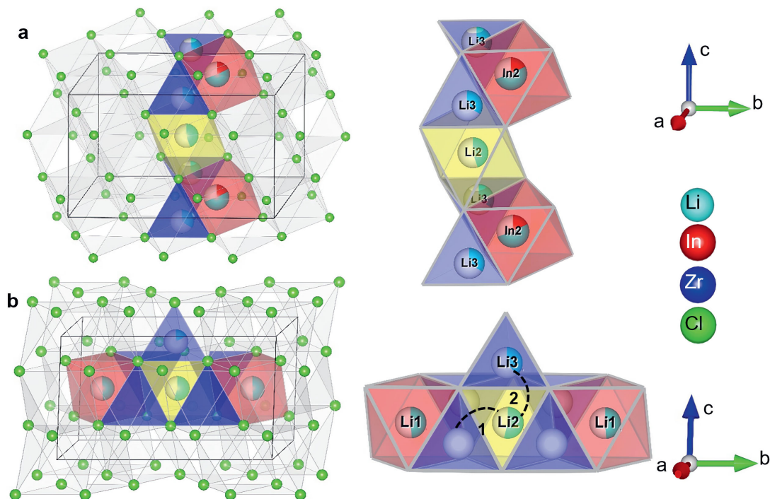
Figure 5.7: Illustration of the possible diffusion pathways in the crystal structure. (a) Diffusion along the c -direction involving the tetrahedral \text{Li3}(8j) site the octahedral \text{Li2}(2c) site and the octahedral \text{In2/Li4}(4g) site (b) Diffusion along the ab plane, illustrating the two different jump processes i.e. 1: jump through the empty tetrahedral site sharing faces with the lithium octahedral sites ( \text{Li1}(4i) , \text{Li2}(2c) ); 2: jump between the \text{Li2}(2c) octahedral site, the occupied tetrahedral \text{Li3}(8j) site and can continue along the \text{In2/Li4} site, as in (a). Diffusion in the M-layer in the ab -plane has similar possible diffusion paths, but with the \text{In1}(2a) site blocking due to the high In/Zr occupancy, strongly reduces the number of free pathways.
