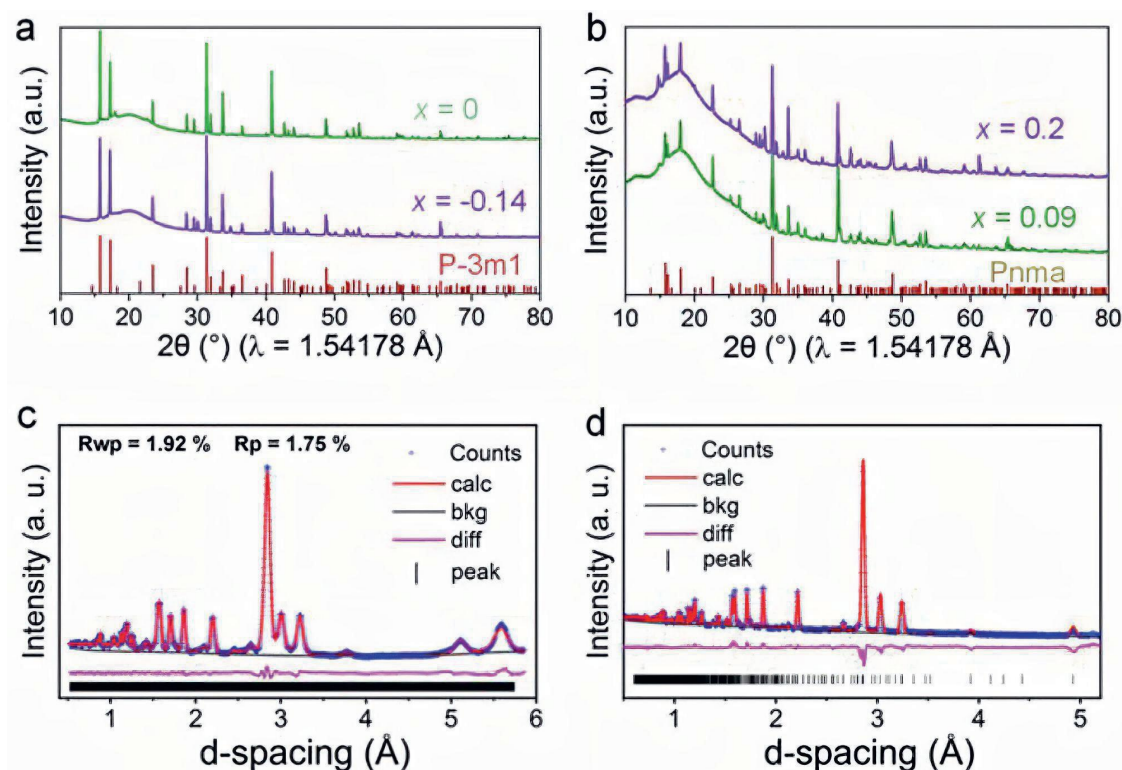
Figure 7.1: XRD and neutron diffraction patterns of the Li-Ho-Cl system. a) XRD patterns of \text{Li}_3\text{HoCl}_6 ( x=0 ) and \text{Li}_{3.42}\text{Ho}_{0.86}\text{Cl}_6 ( x=-0.14 ) samples. Both patterns were indexed to the same space group of P\bar{3}m1 . b) XRD patterns of \text{Li}_{2.4}\text{Ho}_{1.2}\text{Cl}_6 ( x=0.2 ) and \text{Li}_{2.73}\text{Ho}_{1.09}\text{Cl}_6 ( x=0.09 ) samples. The patterns were indexed to the same space group of Pnma . Fitted time-of-flight NPD patterns of c) the \text{Li}_3\text{HoCl}_6 sample, d) the \text{Li}_{2.73}\text{Ho}_{1.09}\text{Cl}_6 sample and the fit resulting from the Rietveld refinement.
