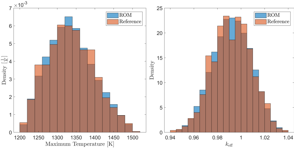
Figure 4.8: Density histograms of the maximum temperature (left) and the multiplication factor k_{eff} (right) by sampling the reduced model with 100,000 points. The distributions of same variables from sampling the reference model with the 1000 testing points are also shown. Note that the histogram is normalized such that the sum of the areas of the bars equals to 1.
