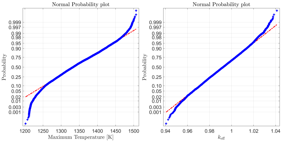
Figure 4.9: Normal probability plots for the maximum temperature (left) and the multiplication factor k_{eff} (right) showing the distribution to be normal within the middle parts but deviating from the normal distribution at the tails.
