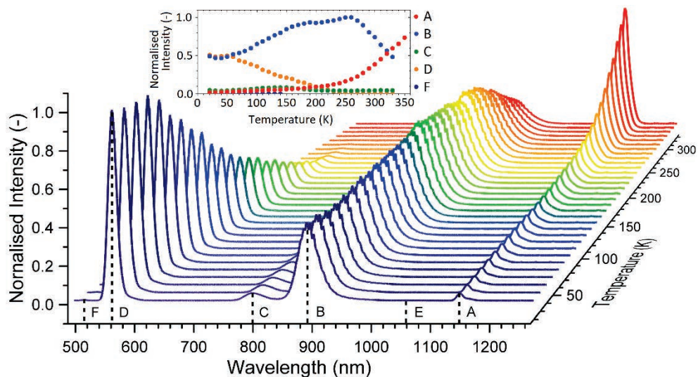
Figure 4.15: 3D-Plot showing the qualitative behaviour of the six Tm^{2+} emissions (A to F) in CsCaI_3:Tm^{2+} over temperature. The complementary inset presents the integrated luminescence signals over temperature and allows a qualitative description of the observed trends. The spectra are corrected for the sensitivity of detection and normalized on the (^3F_4, t_{2g})_{S=3/2} \rightarrow ^2F_{7/2} emission D at 20 K. Photoexcitation occurred into the (^3F_4, t_{2g})_{S=1/2} levels at 455 nm.
