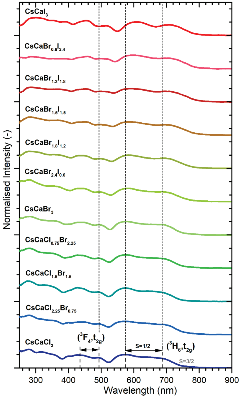
Figure 4.6: Excitation spectra of the CsCa(Cl/Br) 3 :Tm 2+ and CsCa(Br/I) 3 :Tm 2+ samples as acquired on 2 F 5/2 → 2 F 7/2 emission A at 300 K. The lowest energy 4f 12 5d 1 -levels are indicated for CsCaCl 3 :Tm 2+ and undergo a shift towards longer wavelengths upon traversing from Cl→Br→I.
