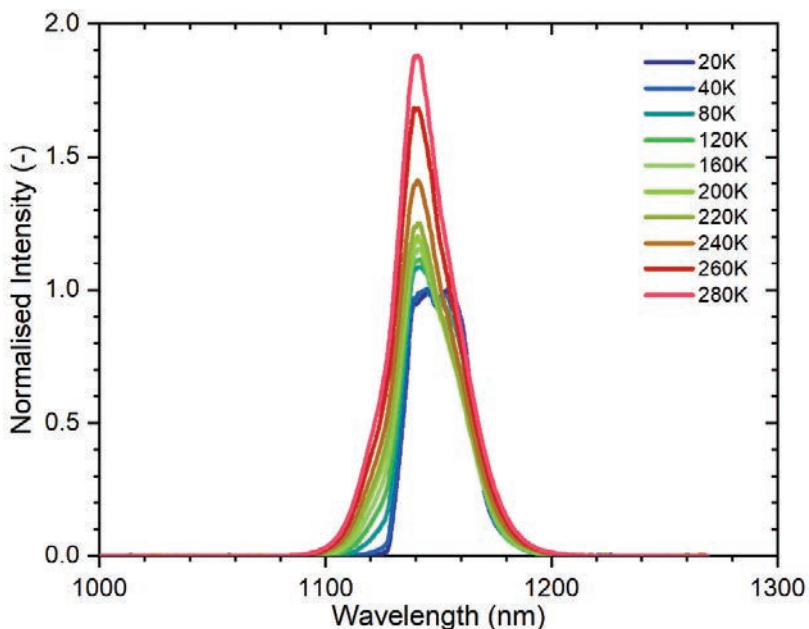
Figure 2.17: The temperature-dependent emission spectra of emission A in NaBr:Tm 2+ as photo-excited at 420 nm. The spectra are normalised on the emission peak at 20 K.
