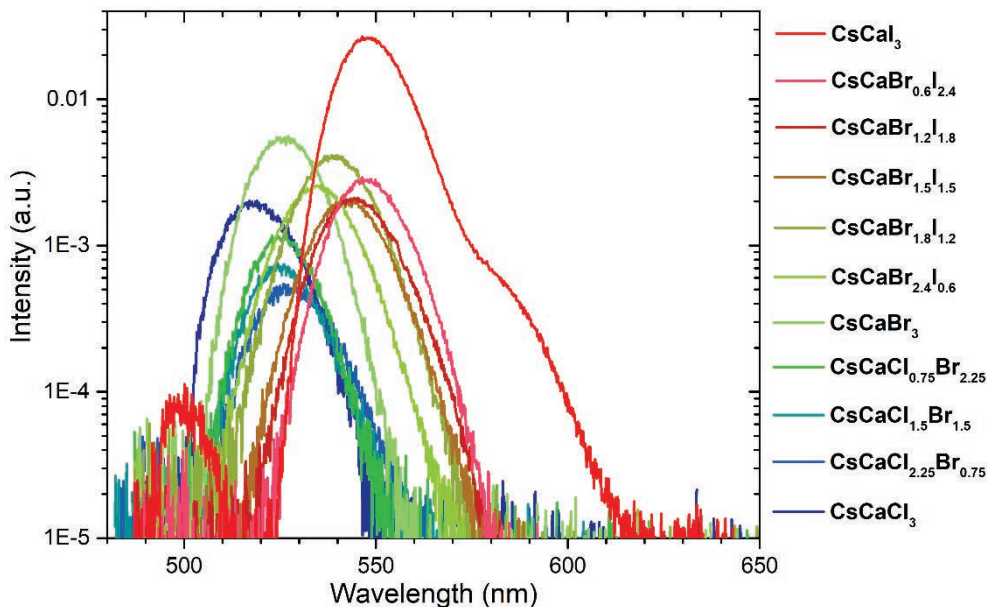
Figure 4.12: Close-up emission spectra of the \text{CsCa}(\text{Cl}/\text{Br})_3\text{Tm}^{2+} and \text{CsCa}(\text{Br}/\text{I})_3\text{Tm}^{2+} samples as centred on emissions D (520-550 nm) and F (500 nm). In analogy to figure 4.10, the spectra are plotted on a log scale. In case of \text{CsCaI}_3\text{Tm}^{2+} a small shoulder is observed for emission D at around 590 nm.
