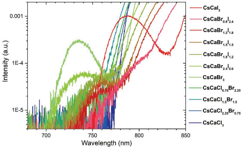
Figure 4.11: Close-up emission spectra of the \text{CsCa}(\text{Cl}/\text{Br})_3\text{Tm}^{2+} and \text{CsCa}(\text{Br}/\text{I})_3\text{Tm}^{2+} samples as centred on emission C (745-790 nm). In analogy to figure 4.10, the spectra are plotted on a log scale.
