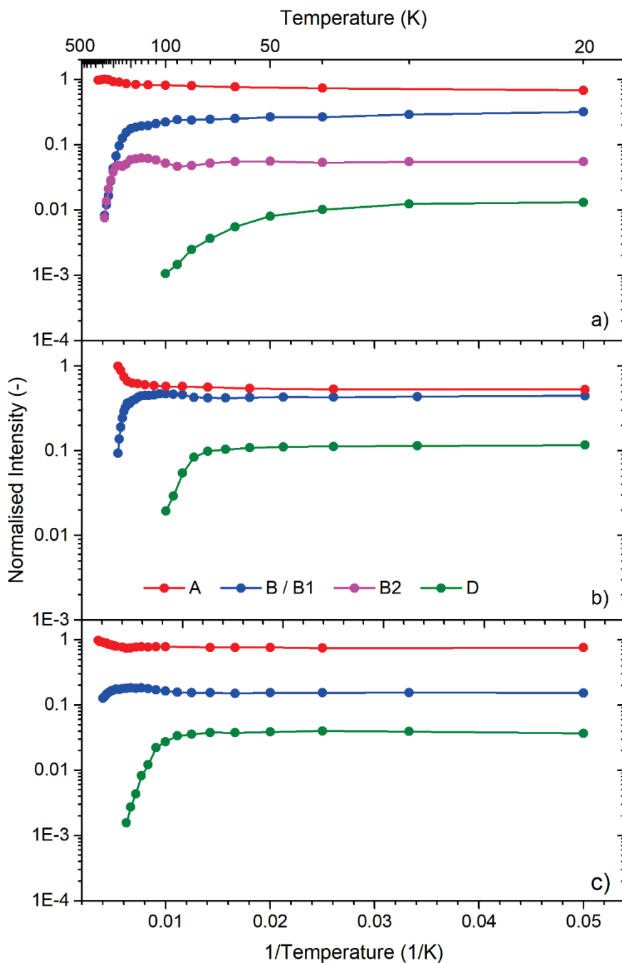
Figure 2.6: Arrhenius plots as based on the integrated emission intensity of the various Tm 2+ emissions. In this figure a) corresponds to NaCl:Tm 2+ , b) to NaBr:Tm 2+ and c) to NaI:Tm 2+ . Photoexcitation occurred at 420 nm, whereas normalisation was performed on emission A at 300 K.
