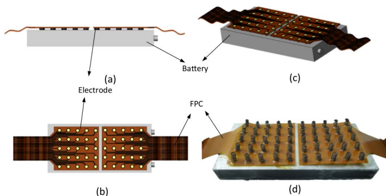
Fig. 3.4: Schematic (a-c) and real (d) representation of a Li-ion battery with ERT sensors shown in various viewing angles. The yellow dots indicate the sense electrodes, which are attached to a so-called flexible printed circuit (FPC), serving as measurement cable. Adopted from Ref. [40].
