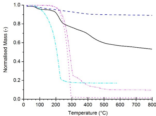
Figure S2: TGA of used Lu(TMHD)3 [---] with the potential precursors as comparison. (Lu(acac) 3 [—], Lu(TMHD) 3 [····], Lu(HMDS) 3 [---] exposed to air during loading and Lu(HMDS) 3 [-.-] loaded under inert conditions.)
