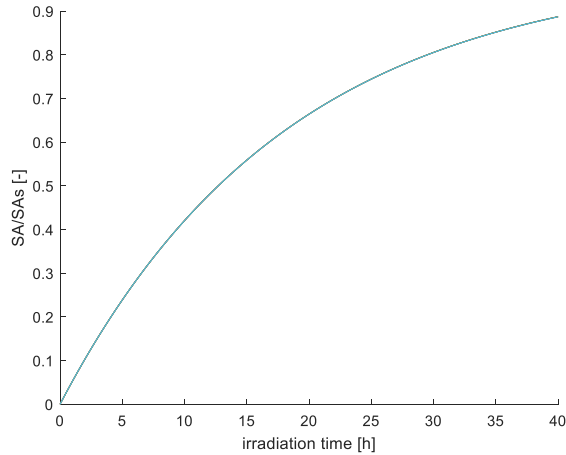
Figure S 2: 64 Cu activity produced normalised over the saturation activity.
