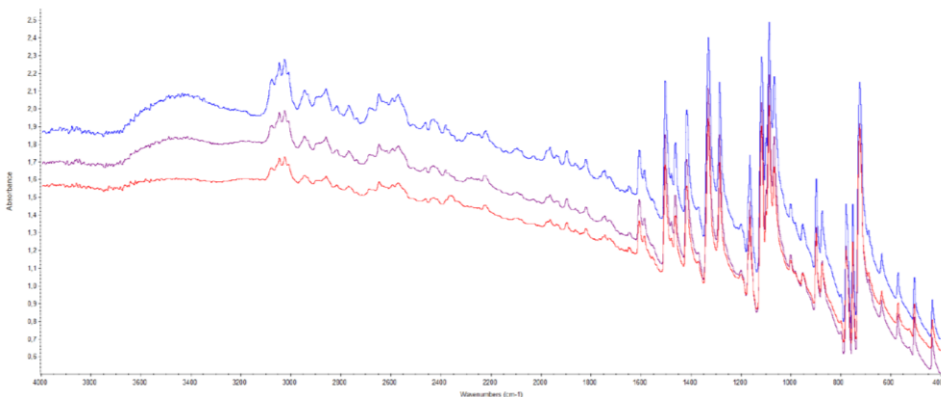
Figure S 3: Result from the FTIR measurements of Cu(II)-phthalocyanine samples receiving an integrated neutron dose of 2.9 \cdot 10^{21} n/m 2 and 1052 kGy (blue) or a gamma dose 386 kGy (purple) compared to a control (non – irradiated) (red).
