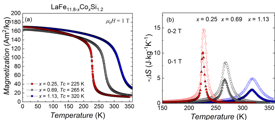
Figure 6.5: Temperature dependent magnetization (a) for LaFe 11.8-x Co x Si 1.2 ( x = 0.25, 0.69 and 1.13 ) compounds measured in a magnetic field of \mu_0 H = 1 T and magnetic entropy change (b) for 1 T (filled symbols) and 2 T (open symbols).
