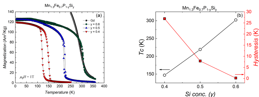
Figure 4.4: Magnetisation as a function of temperature in an applied magnetic field of \mu_0 H = 1 \text{ T} (a) together with the derived Curie temperature T_C and the thermal hysteresis \Delta T_{\text{hys}} as a function of the Si content (b) for the \text{Mn}_{1.3}\text{Fe}_{0.7}\text{P}_{1-y}\text{Si}_y ( y = 0.4, 0.5, 0.6 ) compounds from M-T measurement in 0.01 T external field.
