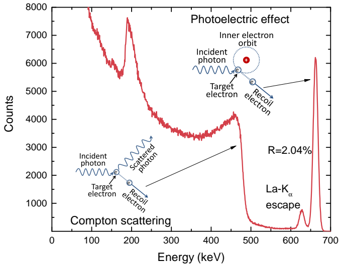
Figure 1.4: Pulse height spectrum of ^{137}\text{Cs} isotope measured with \text{LaBr}_3:\text{Ce,Sr} sample and an Avalanche Photodiode readout. Data reproduced from [7].
