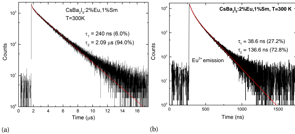
Figure 7.7: a.) X-ray excited luminescence of \text{CsBa}_2\text{I}_5:2\%\text{Eu}^{2+},1\%\text{Sm}^{2+} crystal at 300 K (total emission) b.) with 420 nm optical band-pass filter ( \text{Eu}^{2+} emission only).
