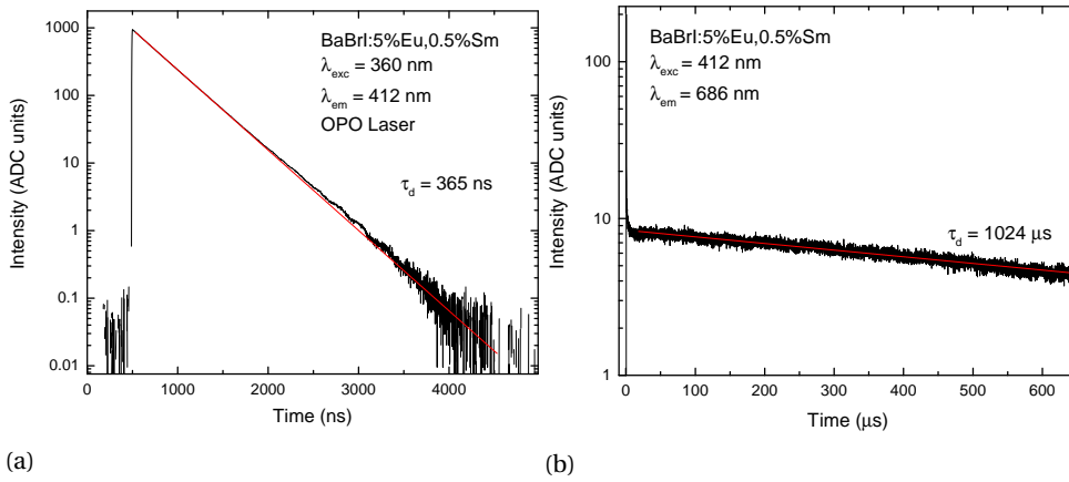
Figure 6.5: a.) Photoluminescence decay profile of BaBrI:5%Eu,0.5%Sm recorded at room temperature using 360 nm optical excitation and emission observed at 412 nm (Eu 2+ 4f-5d transition). b.) Photoluminescence decay profile of BaBrI:5%Eu,0.5%Sm recorded at room temperature using 412 nm optical excitation and emission observed at 686 nm (Sm 2+ 5 D 0 → 7 F 0 transition).
