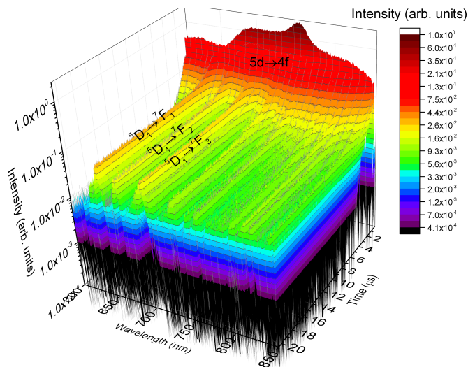
Figure 6.7: Time resolved photoluminescence of BaBr:5%Eu,0.5%Sm at 11 K excited at 360 nm with an OPO laser.
