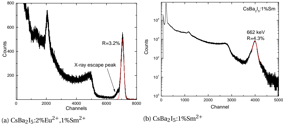
Figure 7.5: Pulse height spectra of ^{137}\text{Cs} measured with a.) \text{CsBa}_2\text{I}_5:2\%\text{Eu}^{2+}, 1\%\text{Sm}^{2+} and b.) \text{CsBa}_2\text{I}_5:1\%\text{Sm}^{2+} single crystals coupled to an APD.
