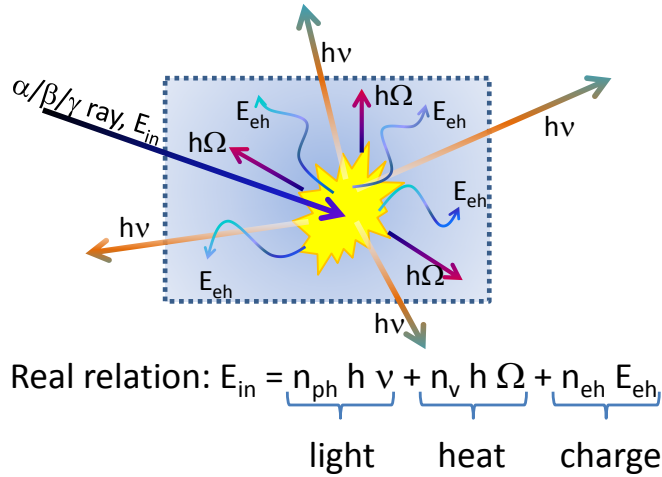
Figure 1.1: Different channels of ionizing radiation energy conversion in matter.
