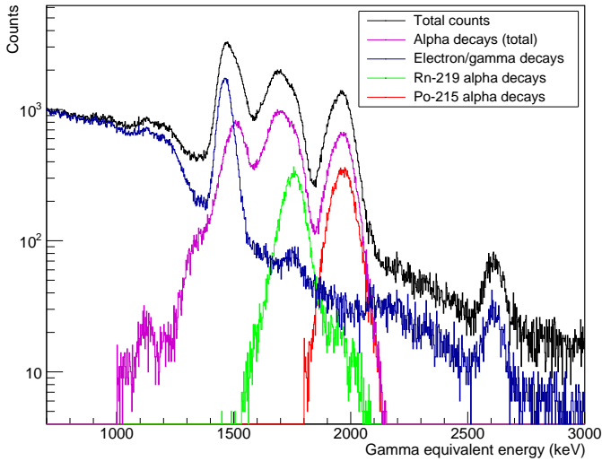
Figure 3.11: Intrinsic activity energy spectrum measured with 2 inch CeBr 3 crystal. Alpha (magenta) and gamma events (dark blue) were separated with PSD, then Radon-219 (green) and Polonium-215 (red) peaks were separated using time-amplitude analysis (colour online).
