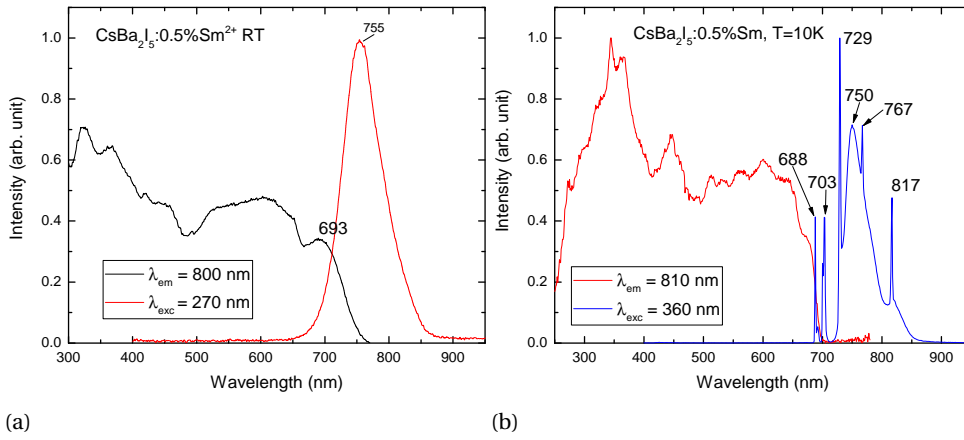
Figure 7.2: Photoluminescence emission and excitation spectra of CsBa 2 I 5 :0.5%Sm 2+ a) at room temperature and b) at 10 K measured with a xenon lamp excitation and a Hamamatsu R7600U-20 photomultiplier.
