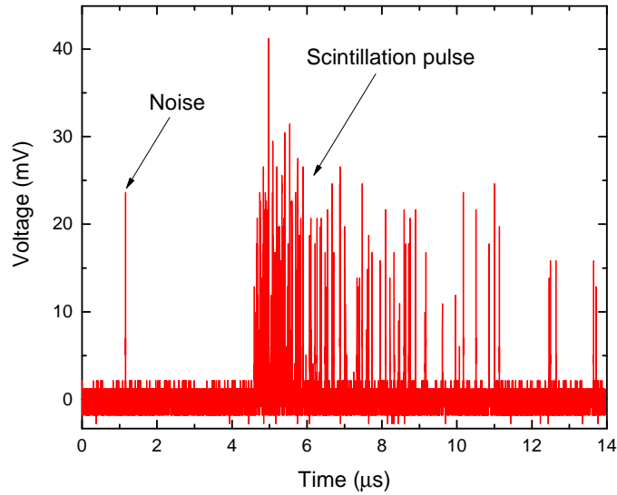
Figure 4.2: Event triggered by a noise spike at around 1 \mu\text{s} with a coincident scintillation pulse starting at around 5 \mu\text{s} .
