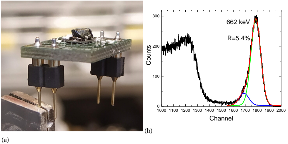
Figure 5.5: CsBa 2 I 5 :Eu,Sm application in nuclear spectroscopy. a) a Si-PM with a CsBa 2 I 5 :Eu,Sm sample mounted on top, b) the pulse height spectrum of CsBa 2 I 5 :Eu,Sm coupled to a SiPM and excited with 662 keV \gamma -rays.
