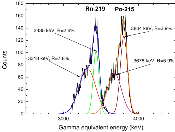
Figure 3.13: Rn-219 and Po-215 alpha peaks measured with internal contamination background in \text{LaBr}_3:\text{Ce},\text{Sr} sample and separated from total background spectrum using pulse shape discrimination and time-amplitude analysis. Asymmetry of alpha peaks is clearly visible.
