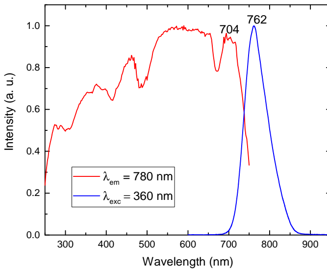
Figure 7.3: Photoluminescence emission and excitation spectra of CsBa 2 I 5 :2%Eu 2+ , 1%Sm 2+ at room temperature measured with a xenon lamp excitation and a Hamamatsu R7600U-20 photomultiplier.
