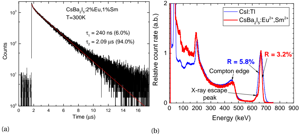
Figure 5.3: a) pulsed X-ray excited scintillation decay, b) pulse height spectra of CsBa 2 I 5 :Eu,Sm and CsI:TI coupled to an APD and excited with 662 keV \gamma -rays.
