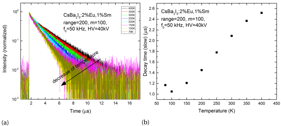
Figure 7.8: X-ray excited luminescence of \text{CsBa}_2\text{I}_5:2\%\text{Eu}^{2+},1\%\text{Sm}^{2+} as a function of temperature. a.) luminescence decay profiles b.) decay time of the dominant (slow) component.
