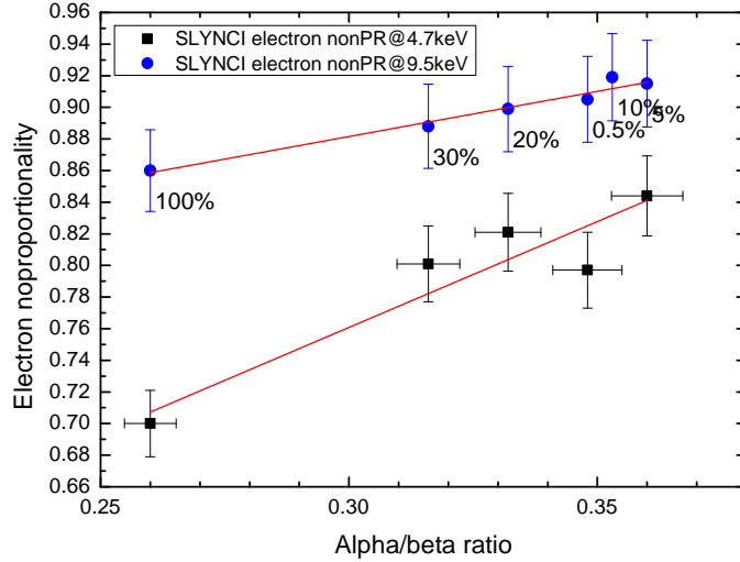
Figure 2.5: Electron nonproportionality of \text{LaBr}_3:\text{Ce} measured with SLYNCI [61] at 4.7 keV and 9.5 keV as a function of the \alpha/\beta ratio, measured at multiple cerium concentrations. Electron response is normalized to 1 at 450 keV, the \alpha/\beta at 662 keV gamma equivalent. Values expressed in percent displayed next to data points show the cerium concentration.
