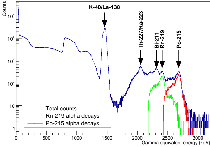
Figure 3.10: Intrinsic activity energy spectrum (dark blue) measured with 3 inch LaBr 3 :Ce (5 mol% of Ce) crystal together with Radon-219 (green) and Polonium-215 (red) peaks separated using amplitude-time analysis (colour online).
