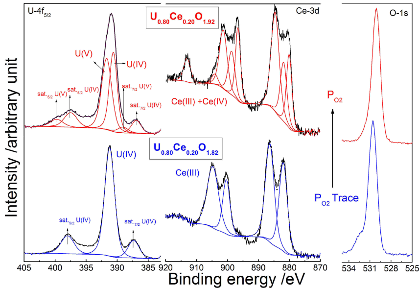
Figure 4.3: U- 4f , Ce- 3d and O- 1s of U_{0.80}Ce_{0.20}O_x Oxide, effect of PO_2 increase during co-deposition. Peaks were deconvoluted using Shirley background correction and the Gaussian-Lorentzian function
