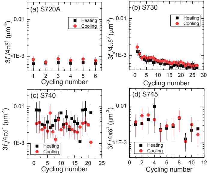
Fig. 4.12. Evolution of the number density of ferrite grains 3f_\alpha/4\pi\delta^3 as a function of the cycling number. The sample name indicates the average temperature during cycling with a temperature span of \Delta T = 20 K.
