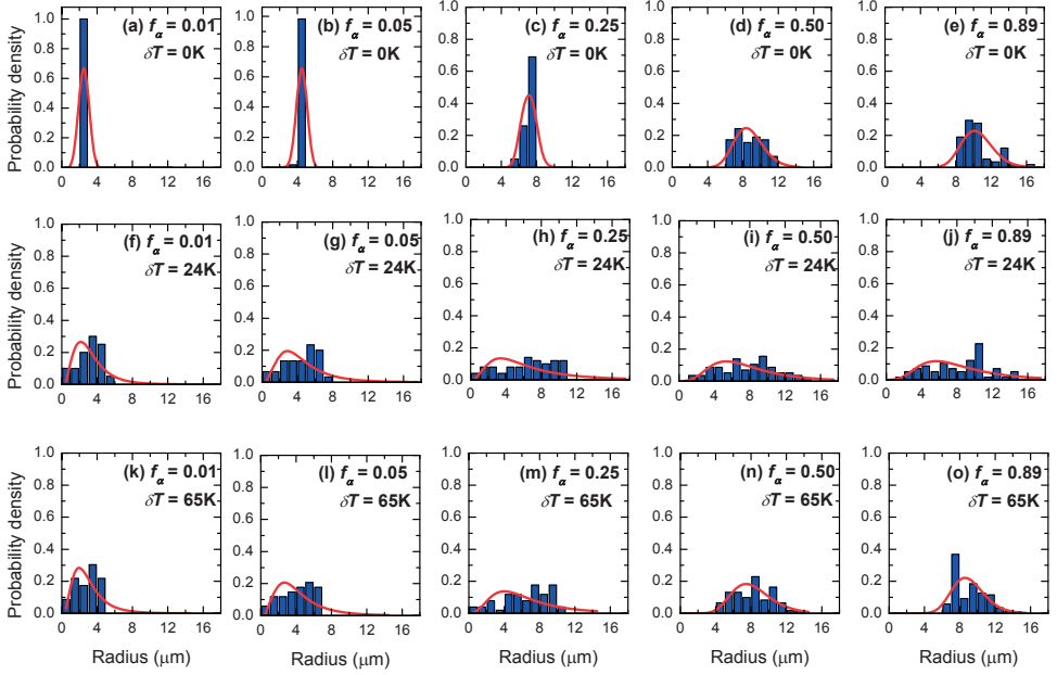
Fig. 2.9. Effect of the nucleation temperature range \delta T on the grain size distribution at a ferrite phase fraction of f_\alpha = 0.01, 0.05, 0.25, 0.50 and 0.89 , respectively. (a)-(e) is modelled with \rho_0 = 1.7 \times 10^{14} \text{ m}^{-3} , \delta T = 0 \text{ K} and M_0 = 1.5 \times 10^{-7} \text{ m}^4 \text{ J}^{-1} \text{ s}^{-1} ; (f)-(j) is modelled with \rho_0 = 1.7 \times 10^{14} \text{ m}^{-3} , \delta T = 24 \text{ K} and M_0 = 3.0 \times 10^{-7} \text{ m}^4 \text{ J}^{-1} \text{ s}^{-1} using SNM and (k)-(o) is modelled with \rho_0 = 2.5 \times 10^{14} \text{ m}^{-3} , \delta T = 65 \text{ K} and M_0 = 3.0 \times 10^{-7} \text{ m}^4 \text{ J}^{-1} \text{ s}^{-1} using CNT. Lognormal fits are shown in solid curves. All simulations show the name transformation kinetics as the dilatometer measurement for a constant cooling rate of 0.4 \text{ K/s} .
