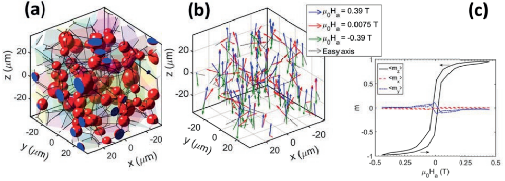
Fig. 3.2. (a) 3D visualization of the microstructure with f = 0.10 , \rho_a = 2.45 \times 10^{14} \text{ m}^{-3} , \langle R \rangle = 4.4 \mu\text{m} and \sigma/\langle R \rangle = 0.25 and (b) the computed magnetisation for each particle illustrated by the orientation of the arrows with easy axis shown in dashed lines. (c) The calculated \langle m_x \rangle , \langle m_y \rangle and \langle m_z \rangle as a function of the applied field (arrows indicate the changing direction of applied field) for a magnetic hysteresis loop.
