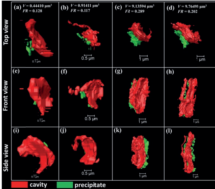
Fig. 7.9. Examples of partially filled creep cavities in Fe-W alloy samples after creep at a temperature of 550 °C and a stress of 140 MPa for a creep time of 0.25t_R . The figure shows representations of four partially filled creep cavities from different angles rendered from high-resolution data with a voxel size of 30 nm. The applied stress is normal to the top view.
