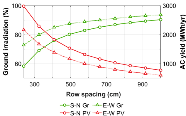
Fig. 6. Sensitivity of average ground irradiation and total AC yield (both annual) to PV topology and spacing. S-N facing topology: 33° tilt, 193° azimuth; while for E-W vertical: 90°, 260°. The energy yield of the reference GMPV is 3 GWh/yr.
