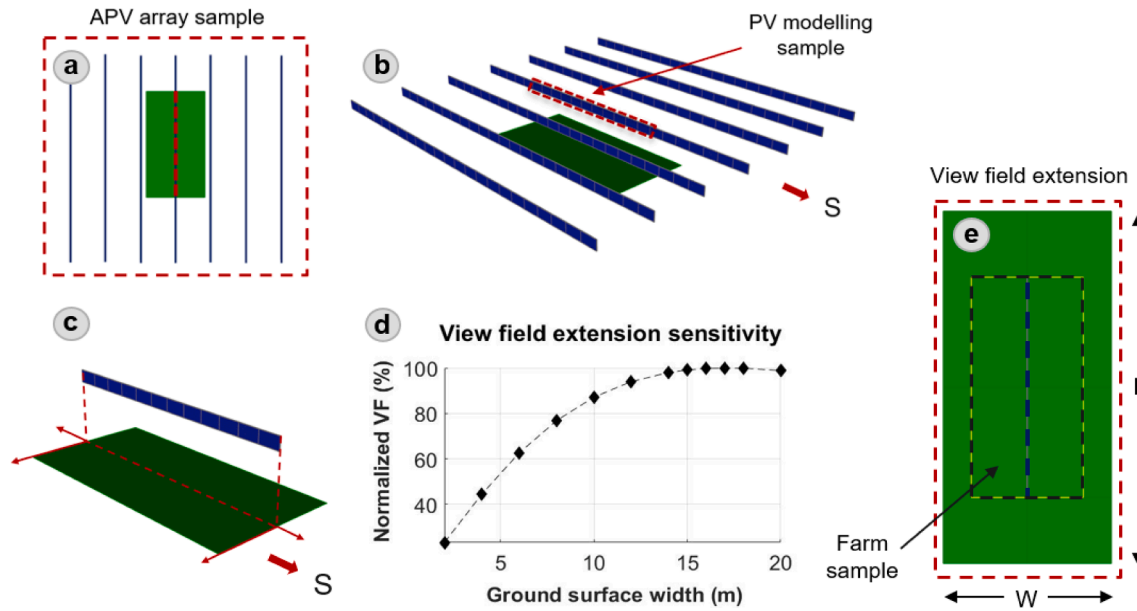
Fig. 4. (a) APV array top view, (b) central string of modules for irradiance modelling, (c) farm sample ( 10 \times 20 \text{ m}^2 ), (d) VF gain for E-W vertical PV topologies, (e) total ground patch ( 15 \times 32 \text{ m}^2 ).
