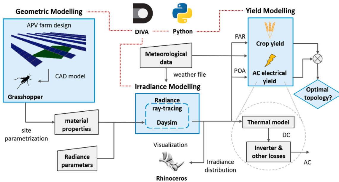
Fig. 2. APV system modelling framework. Rigid lines display the flow of data, while dotted and red lines couple each stage with DIVA through Python. Trapezoids and squares represent inputs and models, respectively. On the bottom right the AC yield model is deconstructed.
